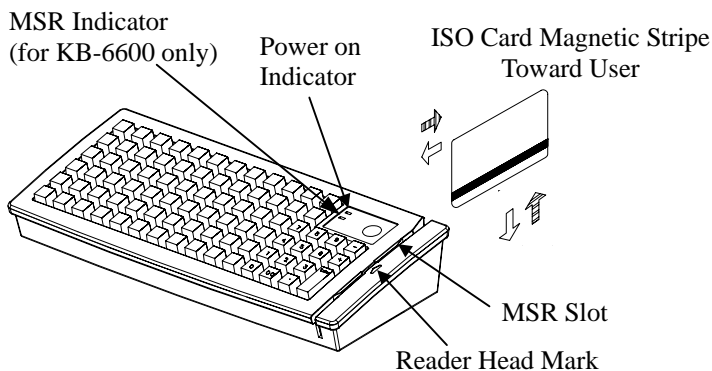
Fig. 4 - 3 Reading magnetic stripe cards of ISO standard
