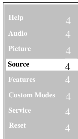
Figure 23: Source Menu
