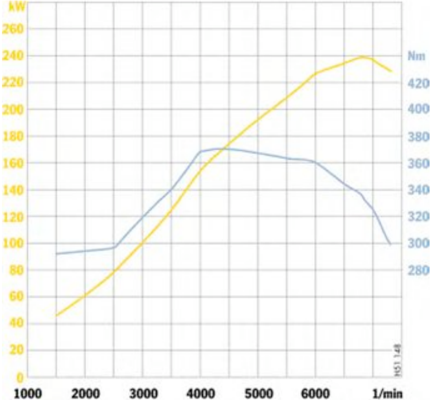
Engine diagram at full power, engine type M96/05
