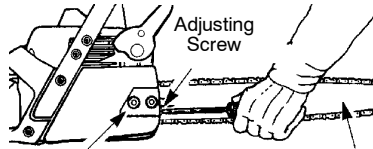
Chain Brake Nuts Guide Bar
