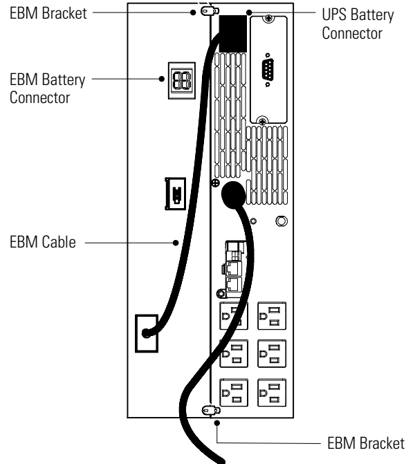
Figure 7. EBM Connections
