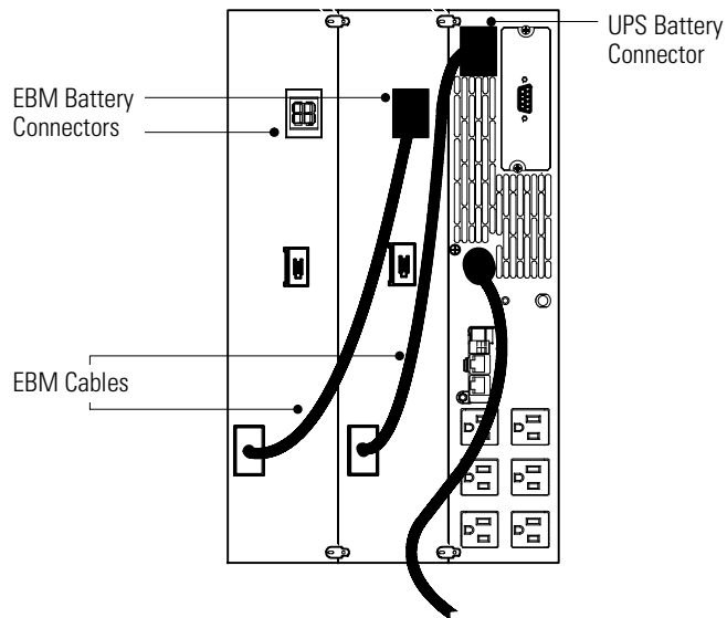
Figure 6. EBM Connections
