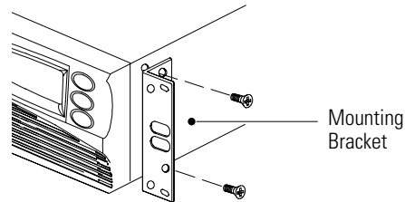
Figure 1. Installing the Mounting Brackets
