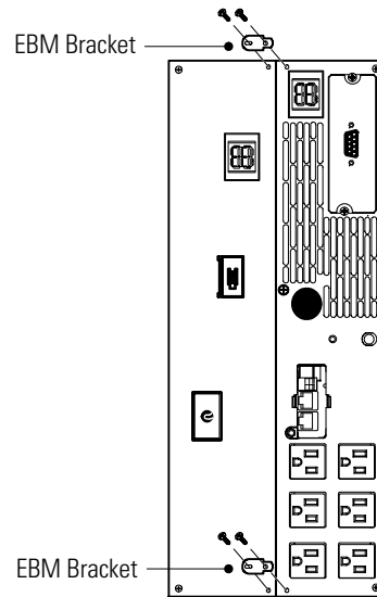
Figure 5. Installing the EBM Brackets
