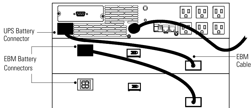
Figure 3. EBM Connections
