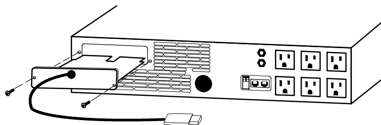
Figure 2. Installing the USB Module
