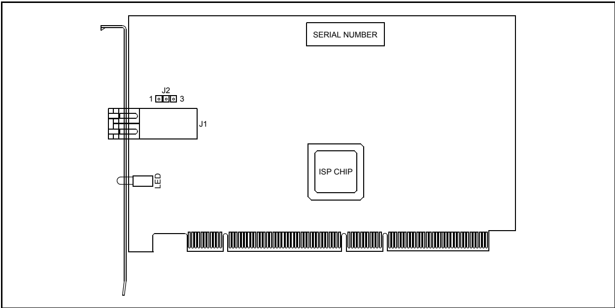
Figure 2-1. QLA2310F HBA Layout
