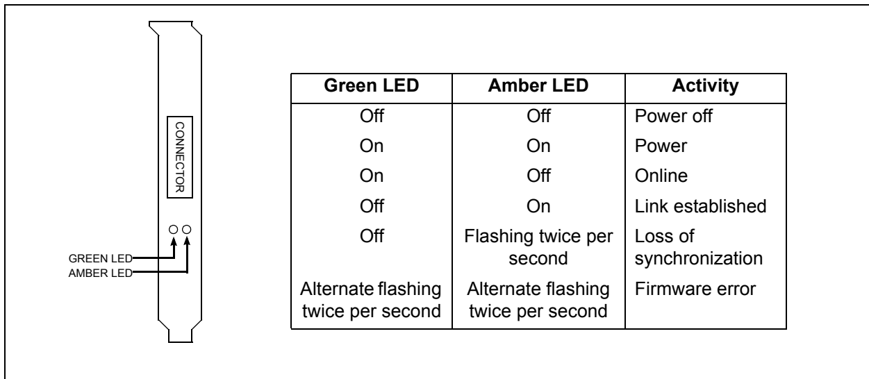
Figure 2-3. QLA2310F/2310FL HBA LED Activity
