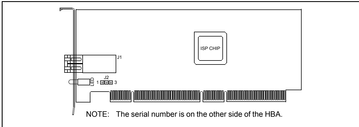
Figure 2-2. QLA2310FL HBA Layout
