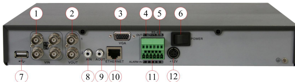
Fig 2-1 QSC26404 Rear Panel
