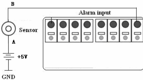
Fig 2.7 Sensor Connection
