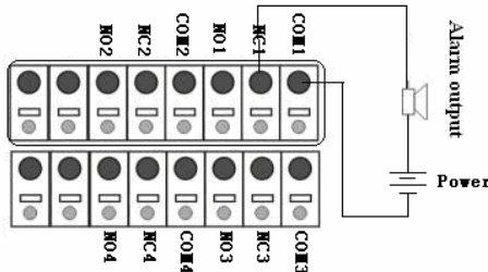
Fig 2.9 Alarm Output Connection
