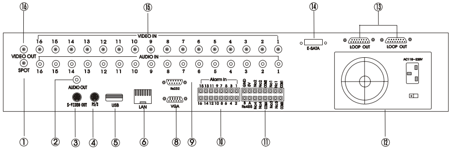
Fig 2.5 Rear Panel for 16-channel DVR
