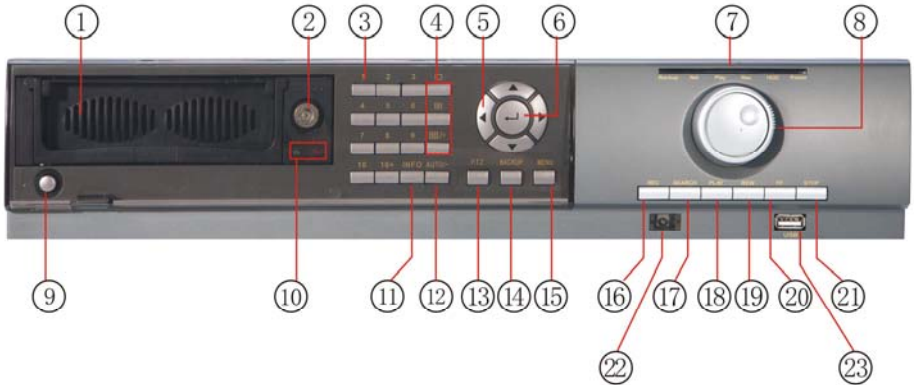
Fig 2.3 Front Panel
