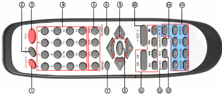
Fig 2.10 Remote Control
