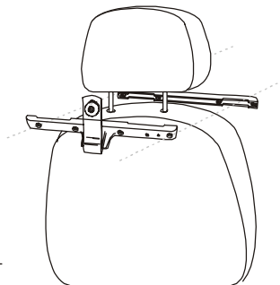
2. HEADREST BRACKET
