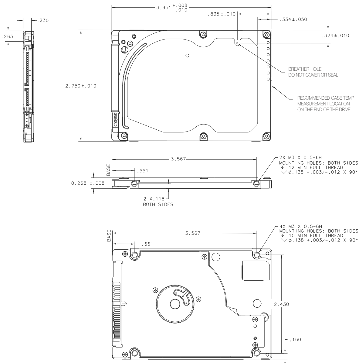
Figure 3 Mounting Dimensions (for standard models)
