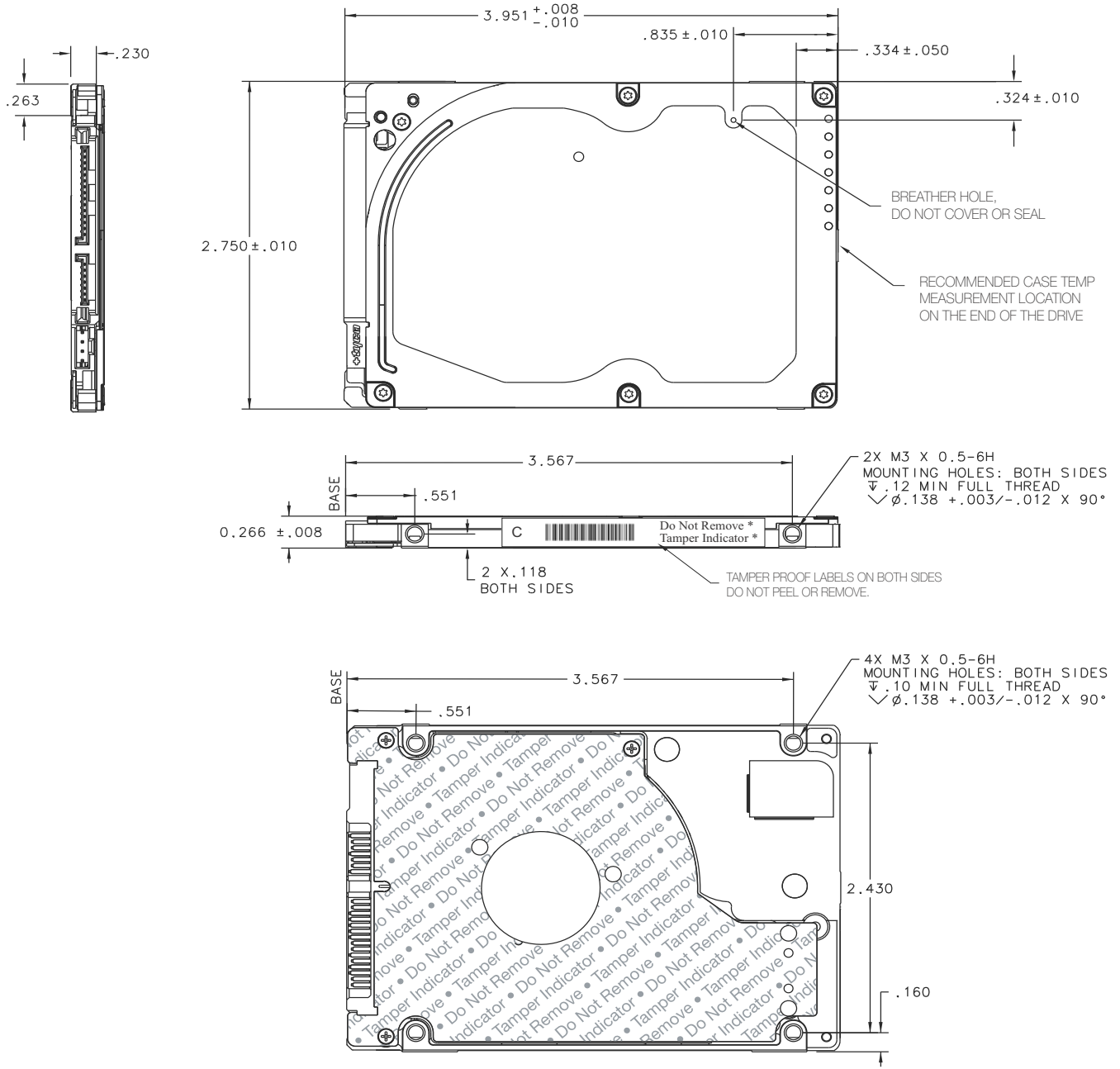
Figure 4 Mounting dimensions (for FIPS 140-2 models)
