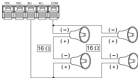
Four 8Ω Speakers
