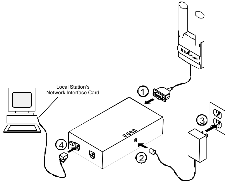
Figure 7: Connecting the DockLINK
