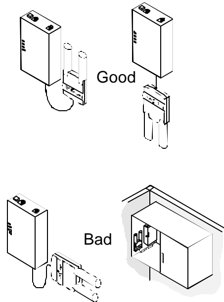
Figure 6: Radio Unit Orientation
