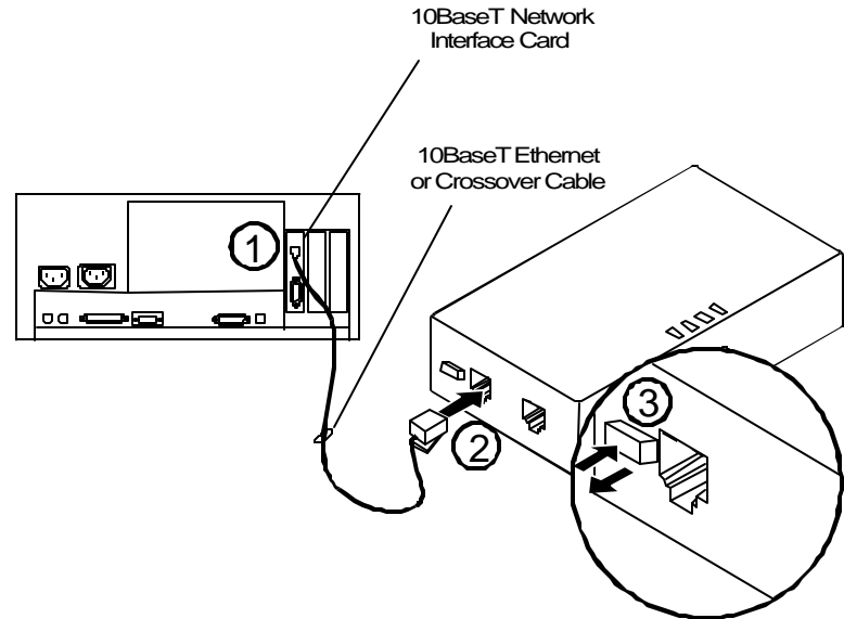
Figure 8: Setting the MDI/MDI-X Switch
