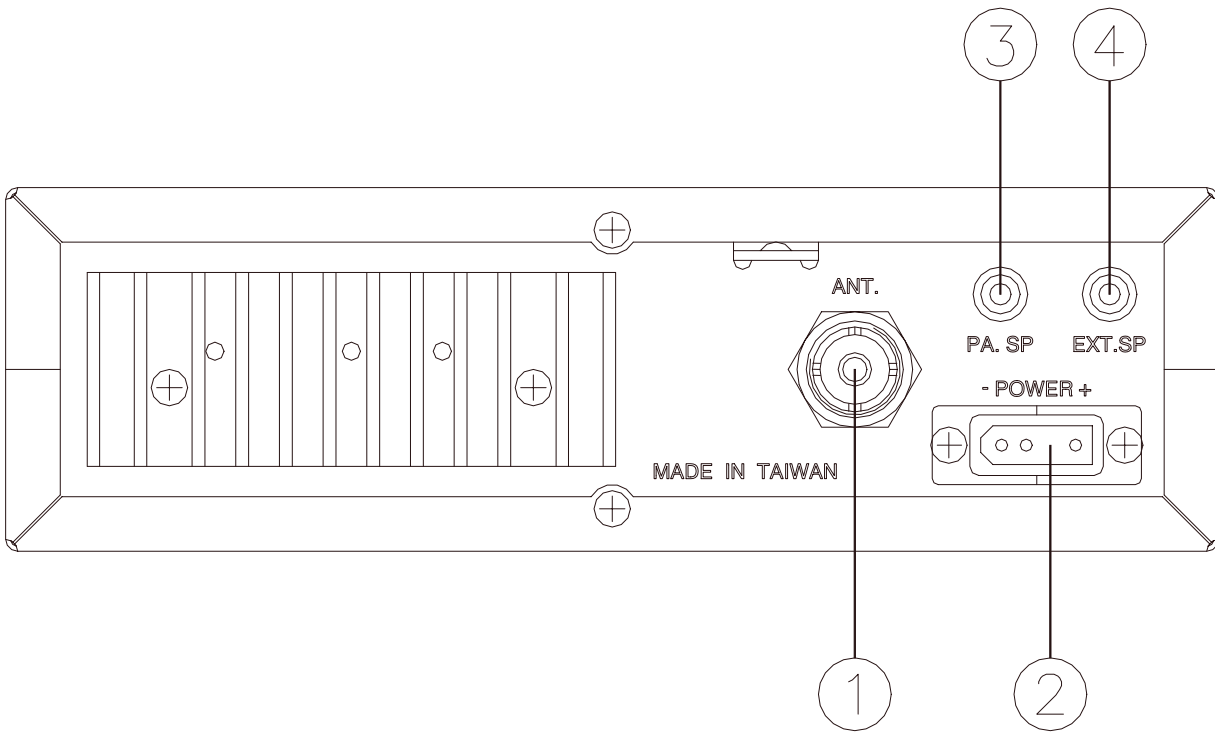
Figure 2-2 Rear Panel
