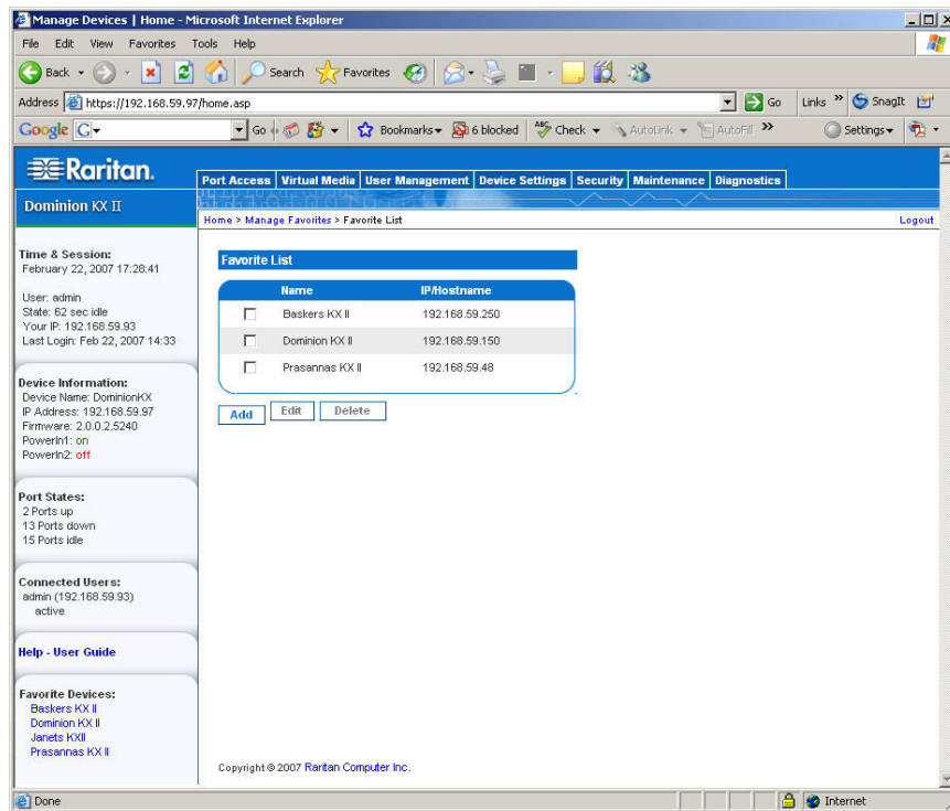
Figure 18: Favorites List
