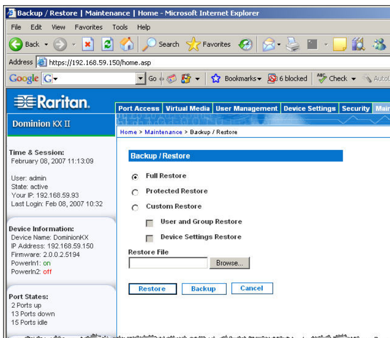
Figure 80: Backup/Restore
