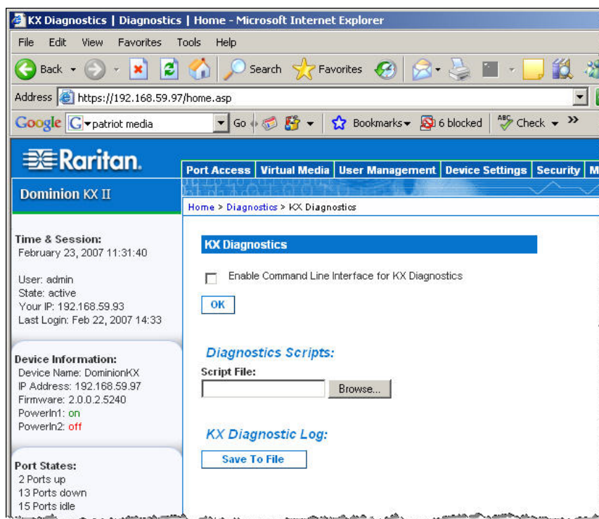
Figure 95: KX Diagnostics
