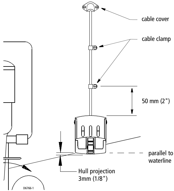
Figure 2-10: Vertical Adjustment and Cable Routing
