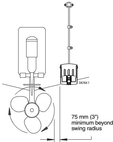
Figure 2-7: Mounting Location on Single Drive Boat
