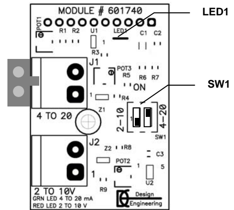
Module set to 4-20 mA mode
