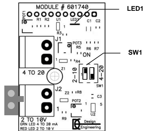
Module set to 2-10 VDC mode
