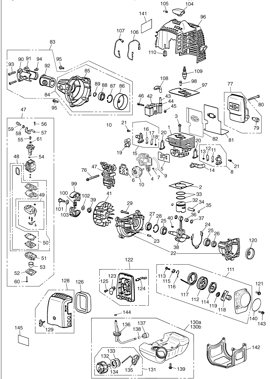
Fig.2 ENGINE UNIT BCZ2610S/BCZ2610S-CA (S/N 70050101 and up)
