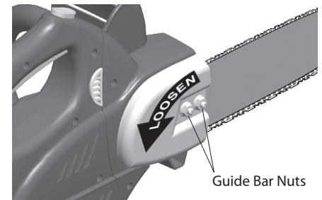
Figure 9 - Loosen Guide Bar Nuts
