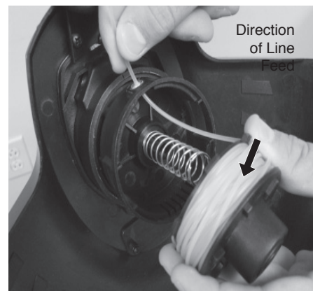
Figure 26 - Inserting line through housing
