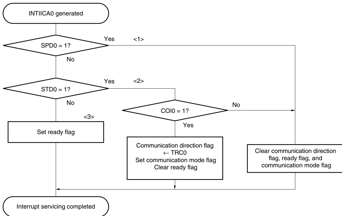
Figure 13-31. Slave Operation Flowchart (2)
