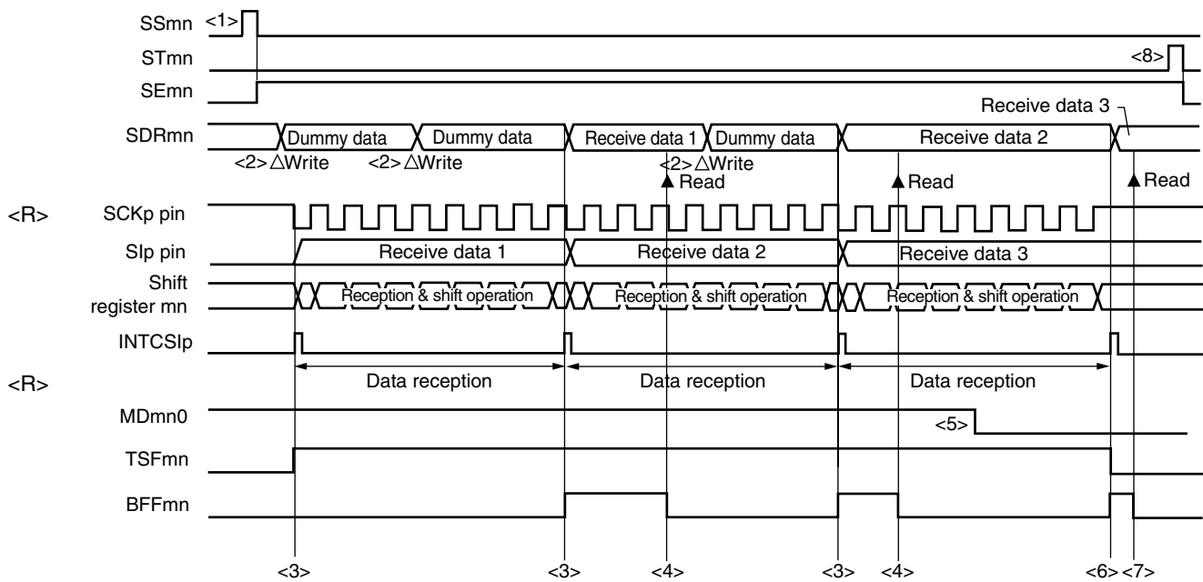
Figure 12-38. Timing Chart of Master Reception (in Continuous Reception Mode) (Type 1: DAPmn = 0, CKPmn = 0)
