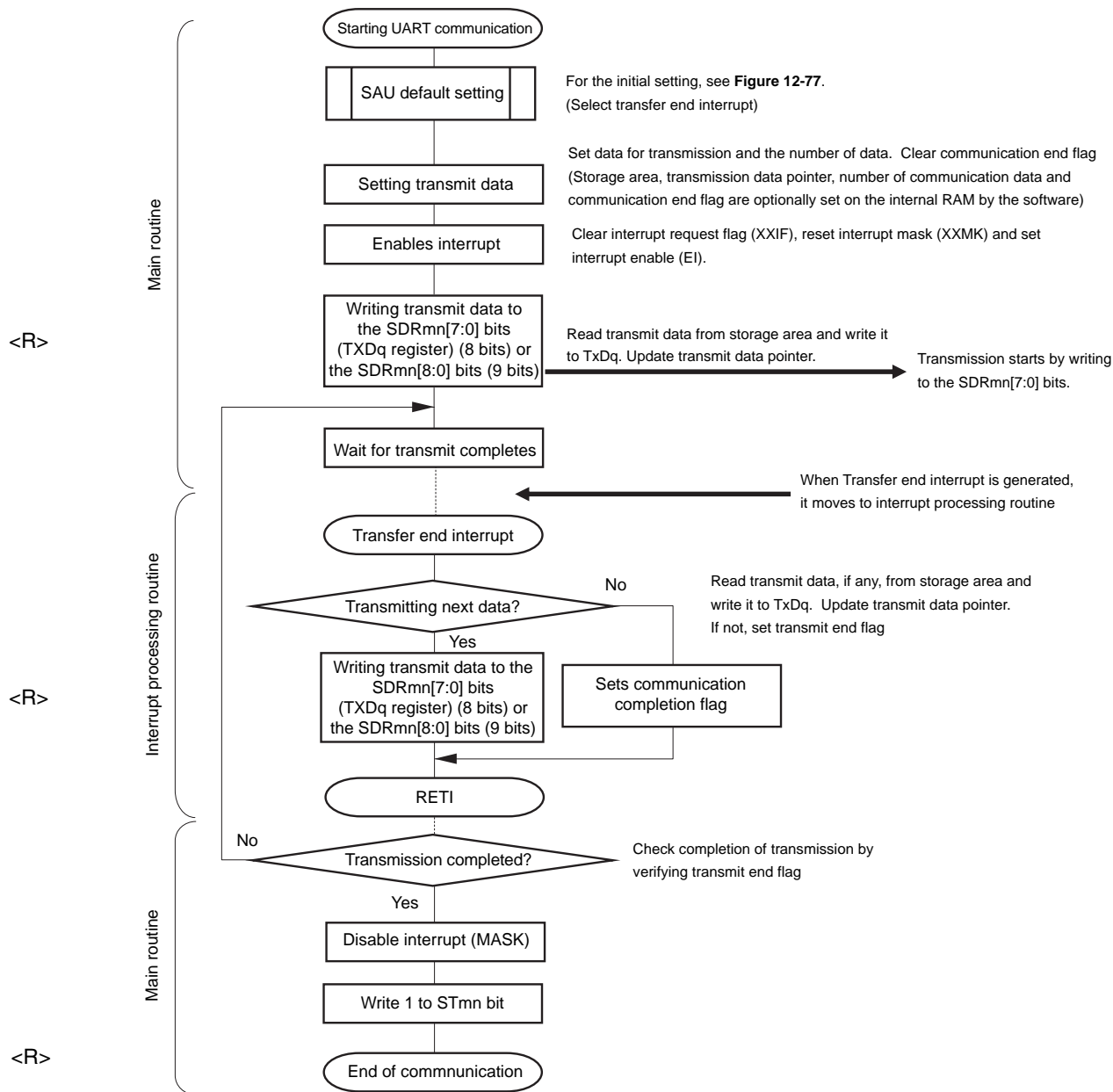
Figure 12-80. Flowchart of UART Transmission (in Single-Transmission Mode)
