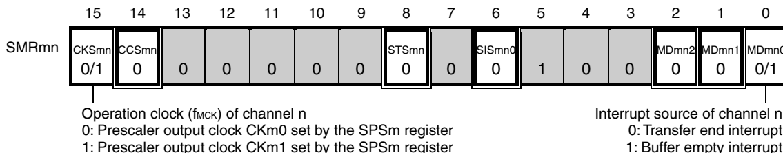
Figure 12-24. Example of Contents of Registers for Master Transmission of 3-Wire Serial I/O (CSI00, CSI01, CSI10, CSI11, CSI20, CSI21) (1/2)
