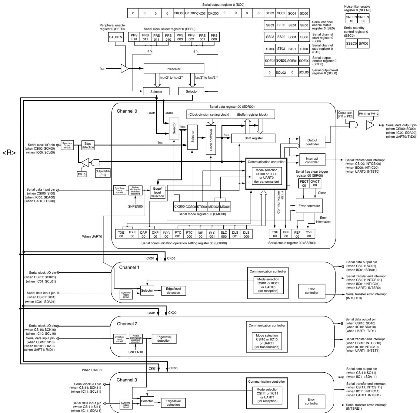
Figure 12-1. Block Diagram of Serial Array Unit 0
