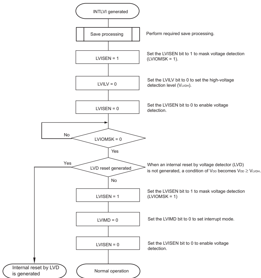
Figure 21-7. Processing Procedure After an Interrupt Is Generated
