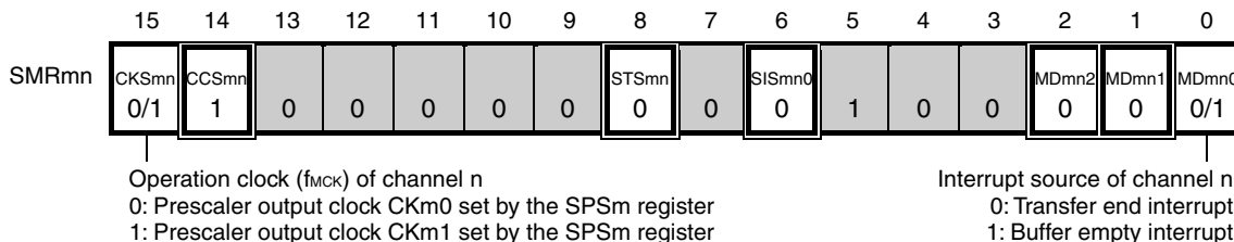
Figure 12-48. Example of Contents of Registers for Slave Transmission of 3-Wire Serial I/O (CSI00, CSI01, CSI10, CSI11, CSI20, CSI21) (1/2)
