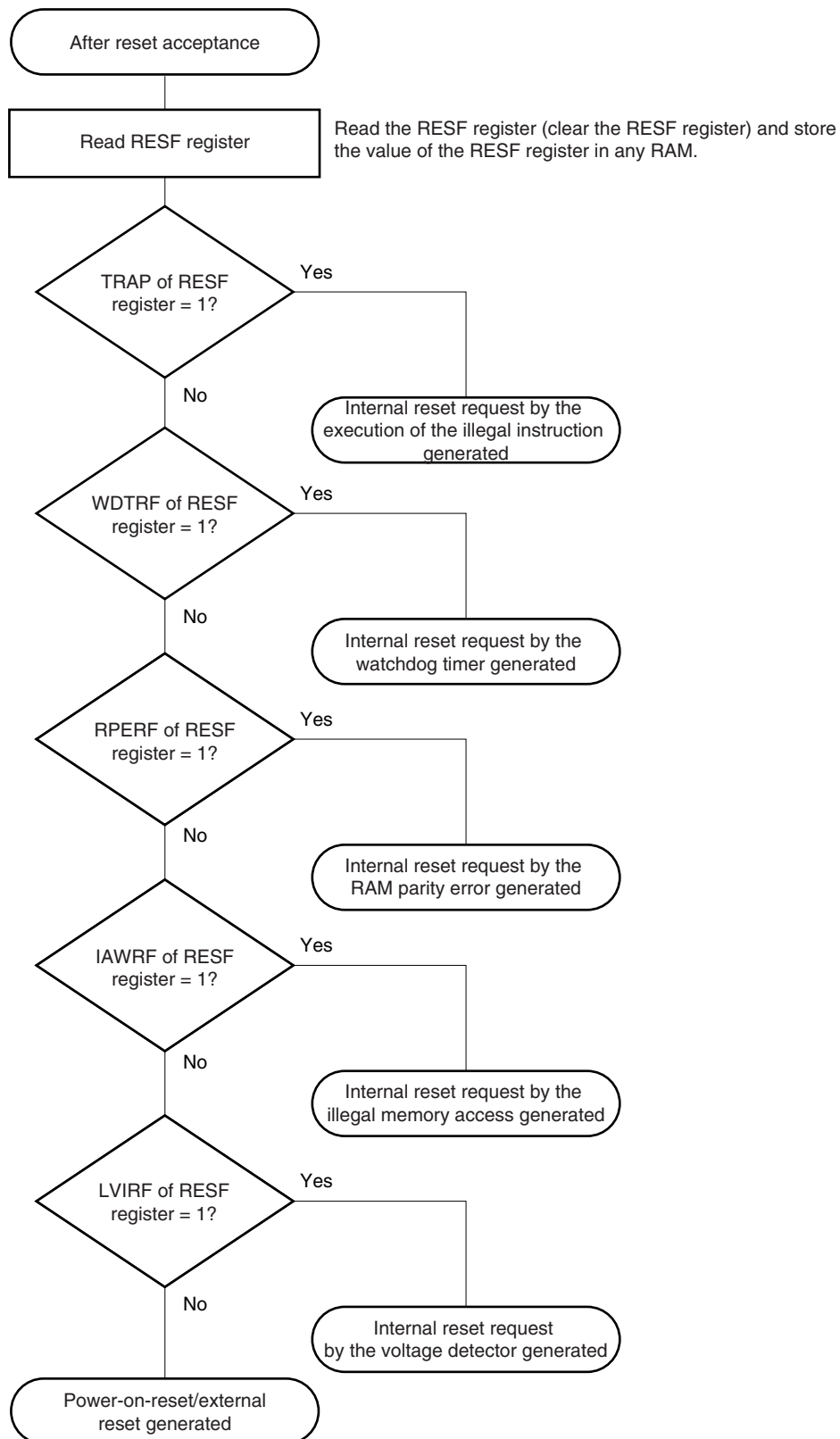
Figure 19-5. Procedure for Checking Reset Source
