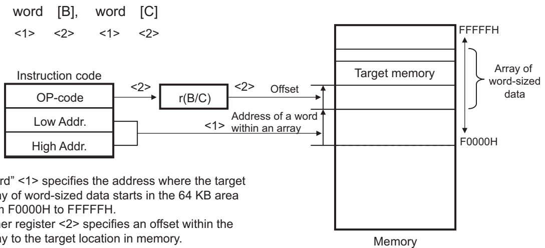
Figure 3-28. Example of word[B], word[C]
