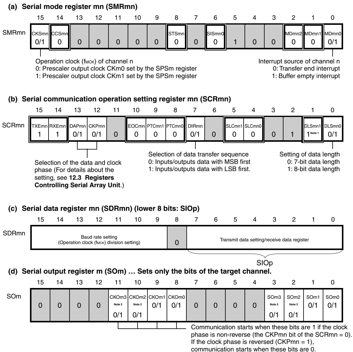
Figure 12-40. Example of Contents of Registers for Master Transmission/Reception of 3-Wire Serial I/O (CSI00, CSI01, CSI10, CSI11, CSI20, CSI21, CSI30, CSI31) (1/2)
