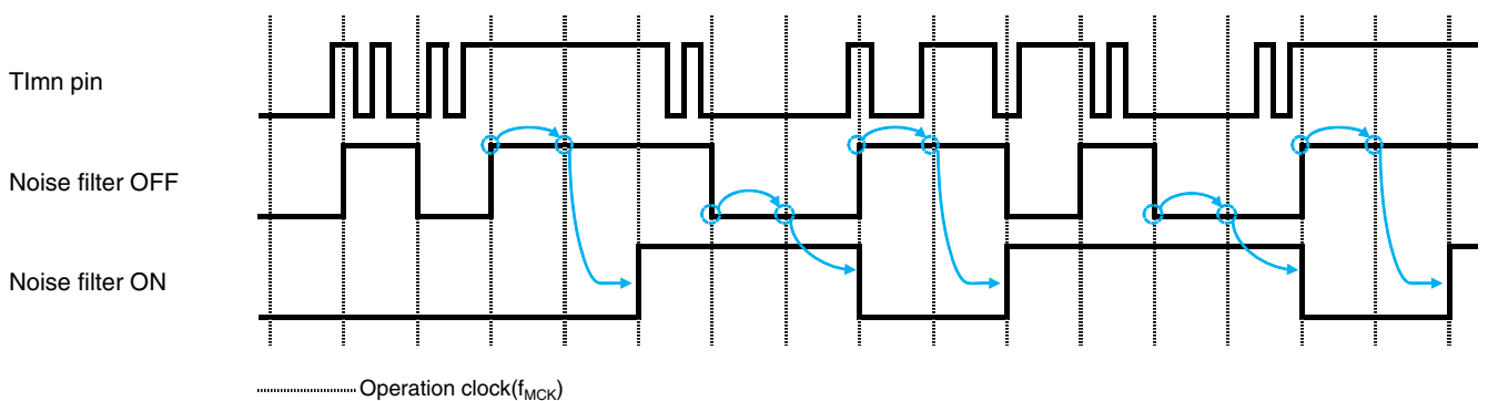
Figure 6-40. Waveform of Sampling Signal Input to Tl mn Pin When Noise Filter Is Enabled and Disabled
