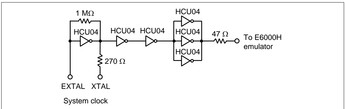
Figure 8 Clock Oscillator
