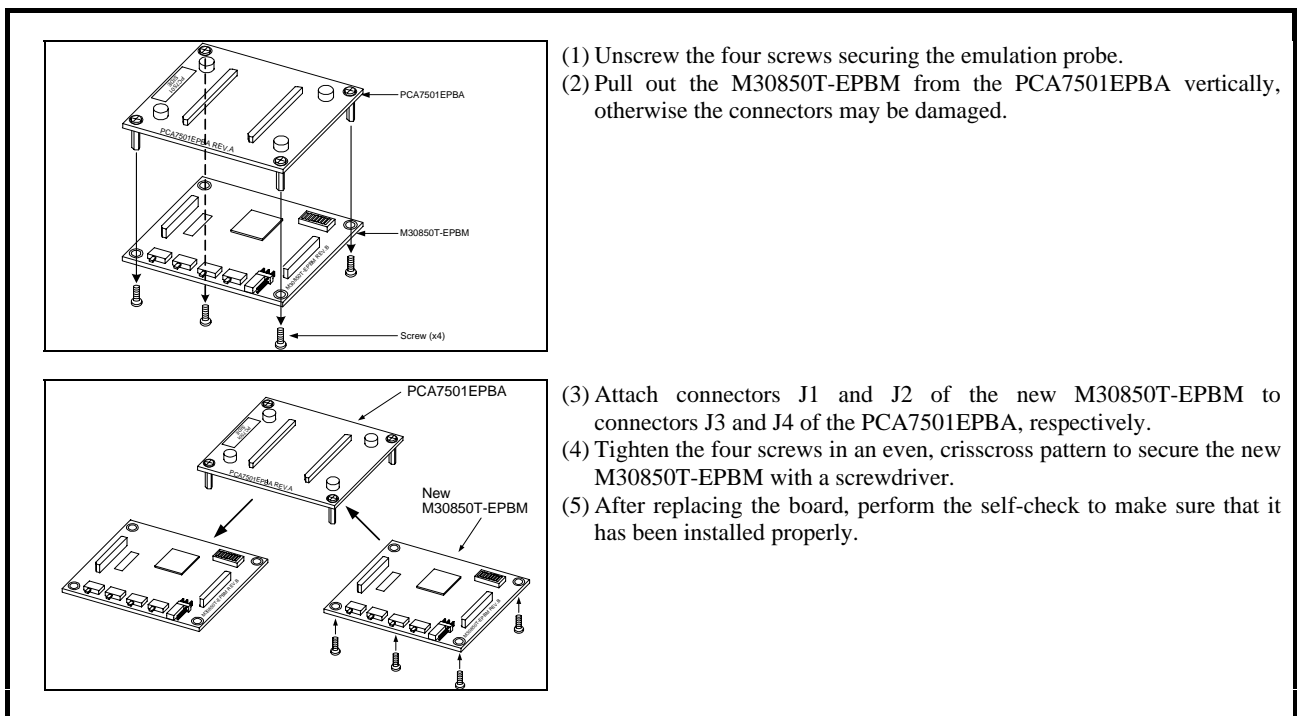
Figure 1 Replacing the MCU board
