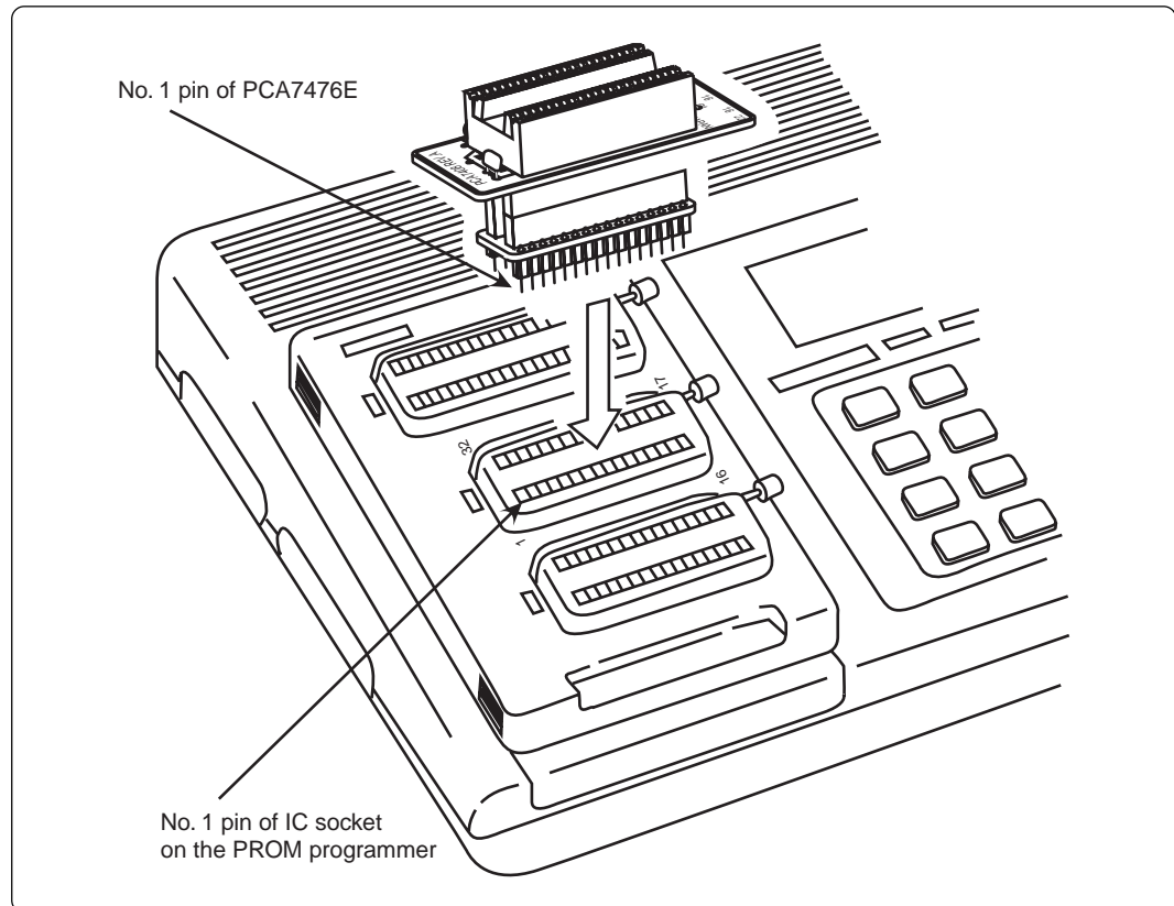
Figure 3.1 Attaching the adapter to the PROM programmer
