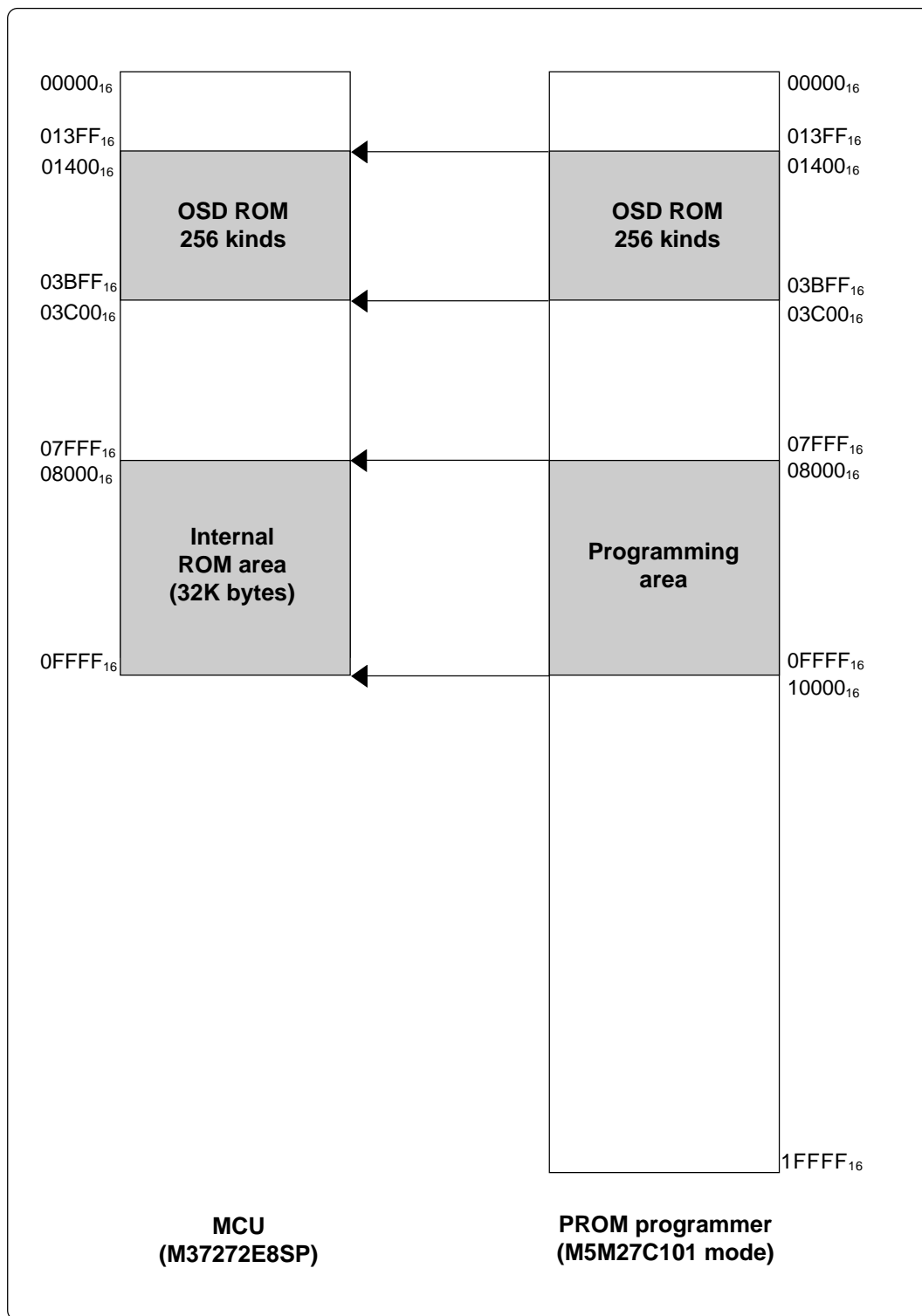
Figure 6.1 Memory map (M37272E8SP)
