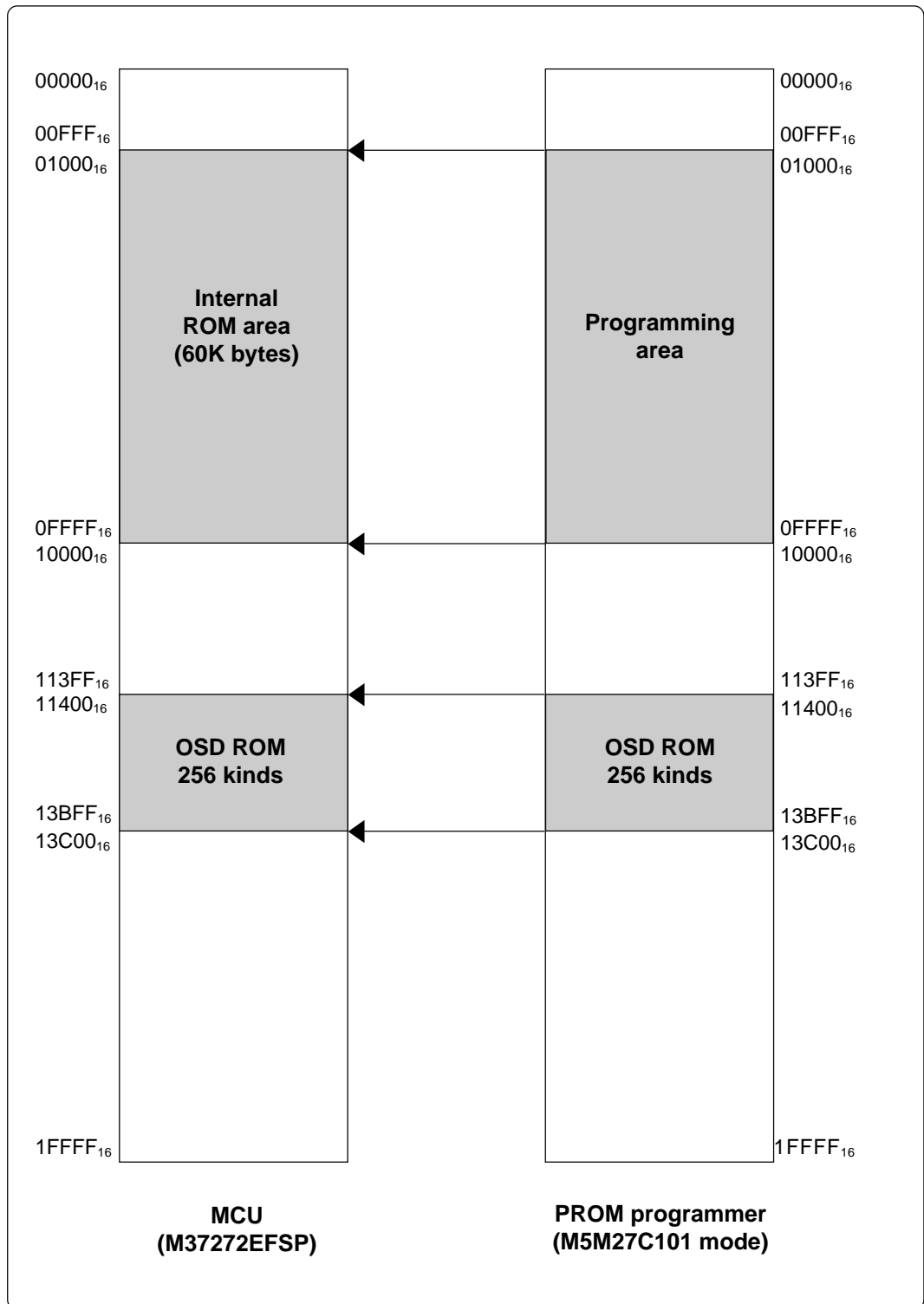
Figure 6.2 Memory map (M37272EFSP)
