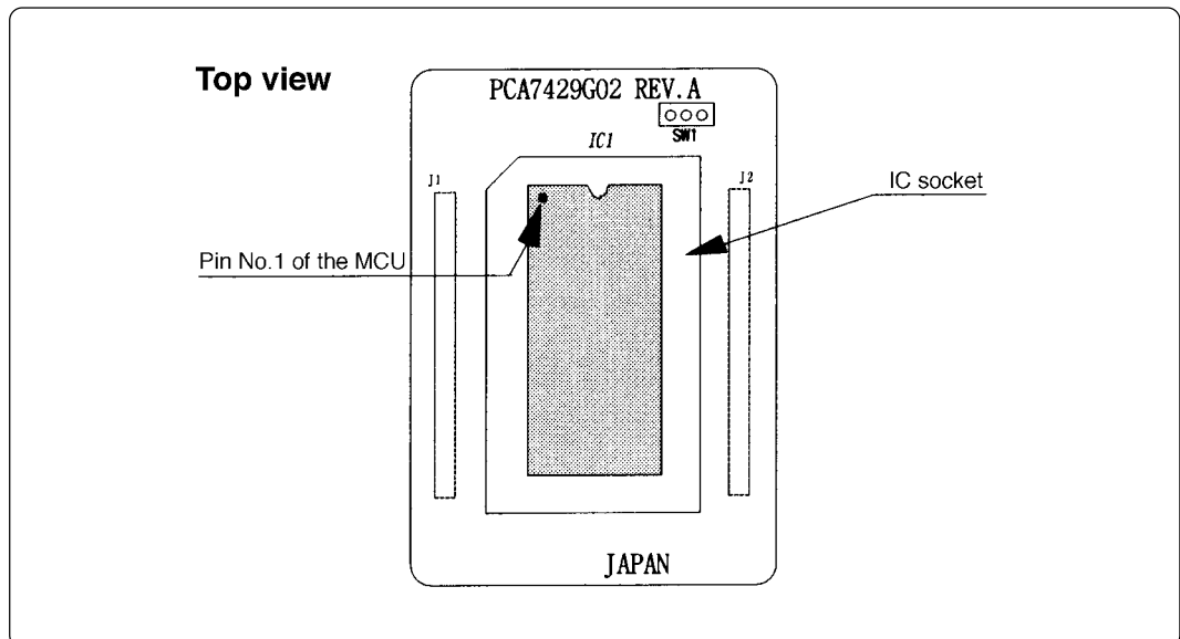
Figure 4.3 Inserting MCU
