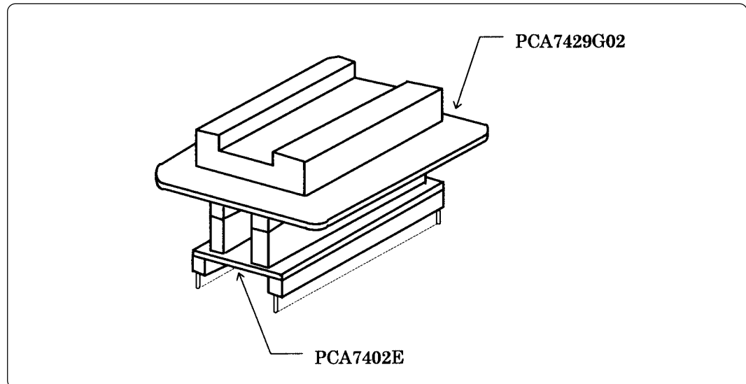
Figure 2.1 External view and constituent parts of PCA7429G02
