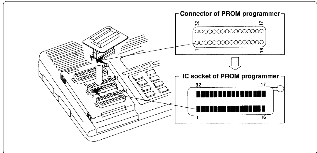
Figure 4.1 Attaching adapter to PROM programmer
