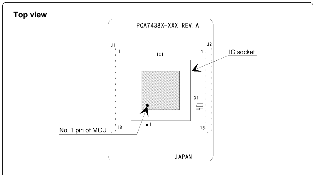
Figure 4.2 Inserting an MCU
