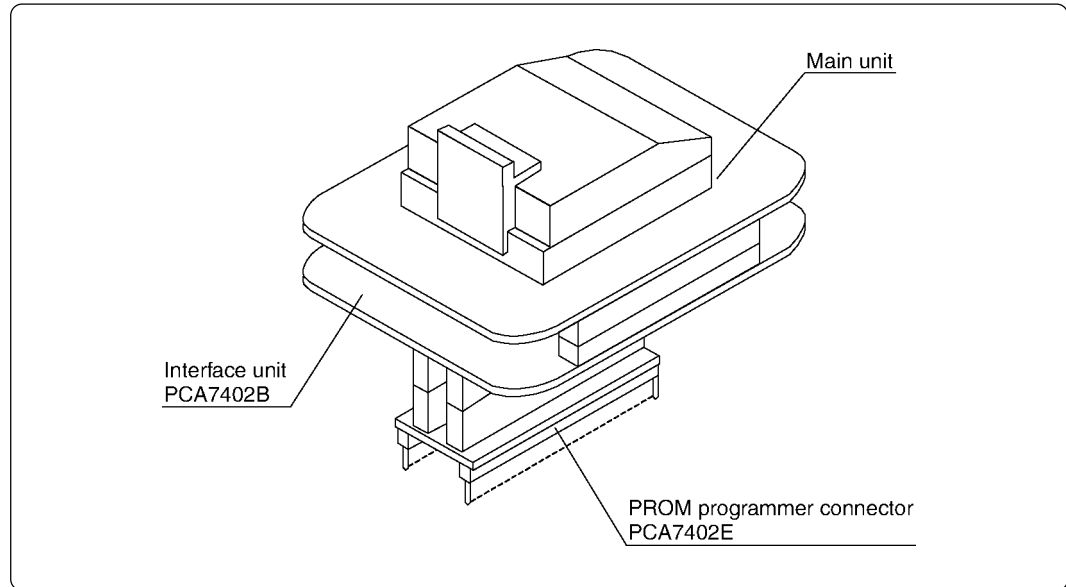
Figure 2.1 External view of PCA7438F-64A/PCA7438H-64A and their constituent parts
