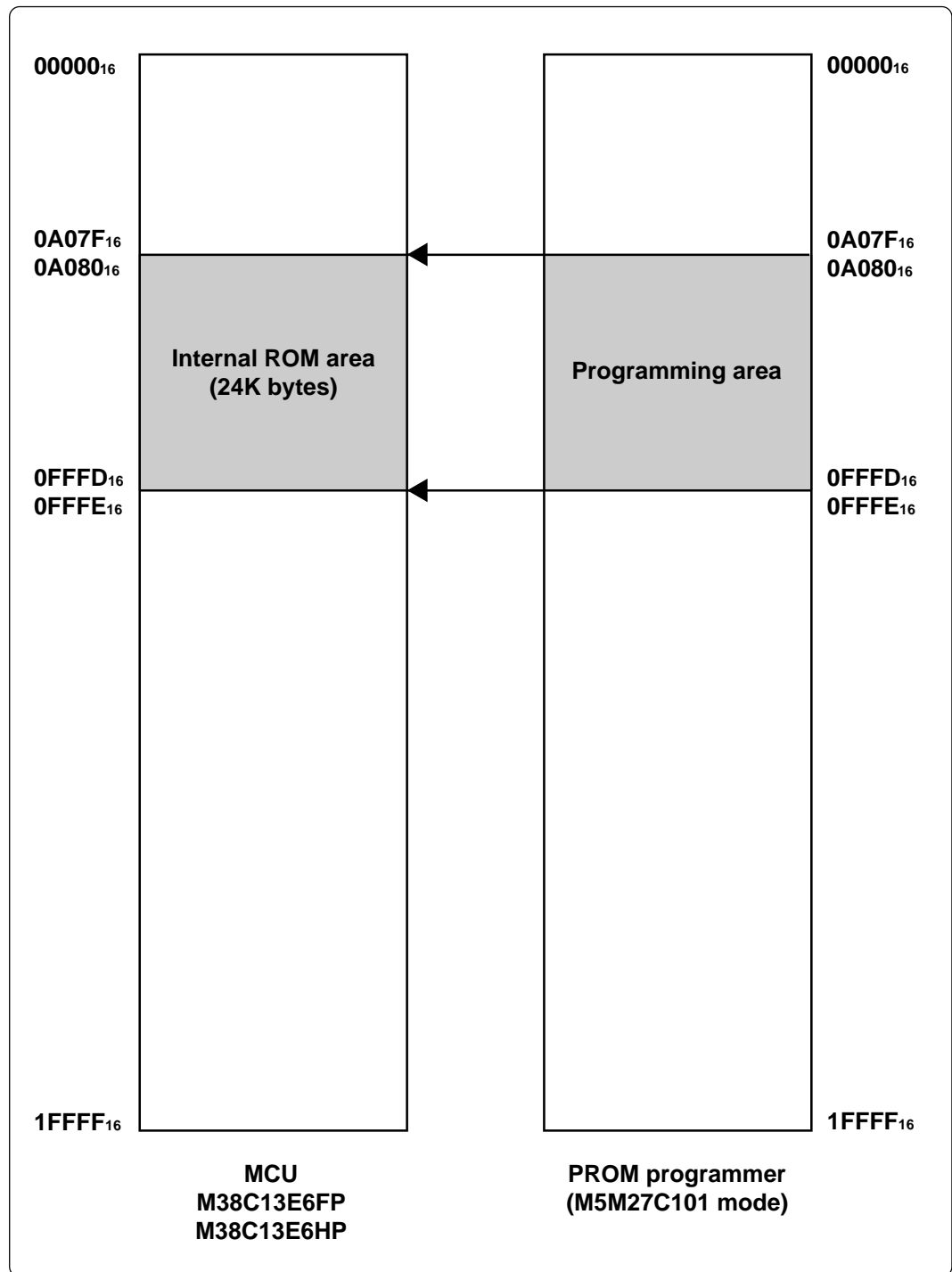
Figure 6.1 Memory map of M38C13E6FP/M38C13E6HP
