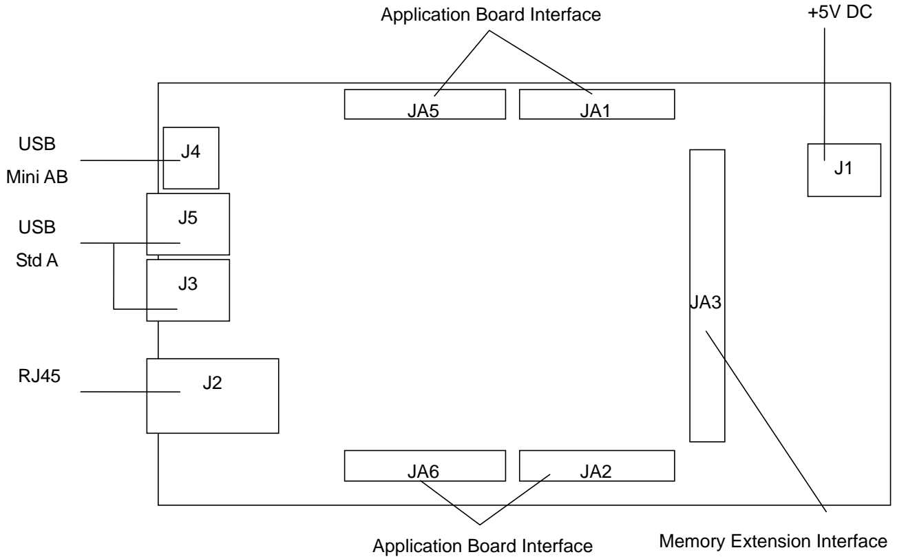
Figure 3-2: Board Layout
