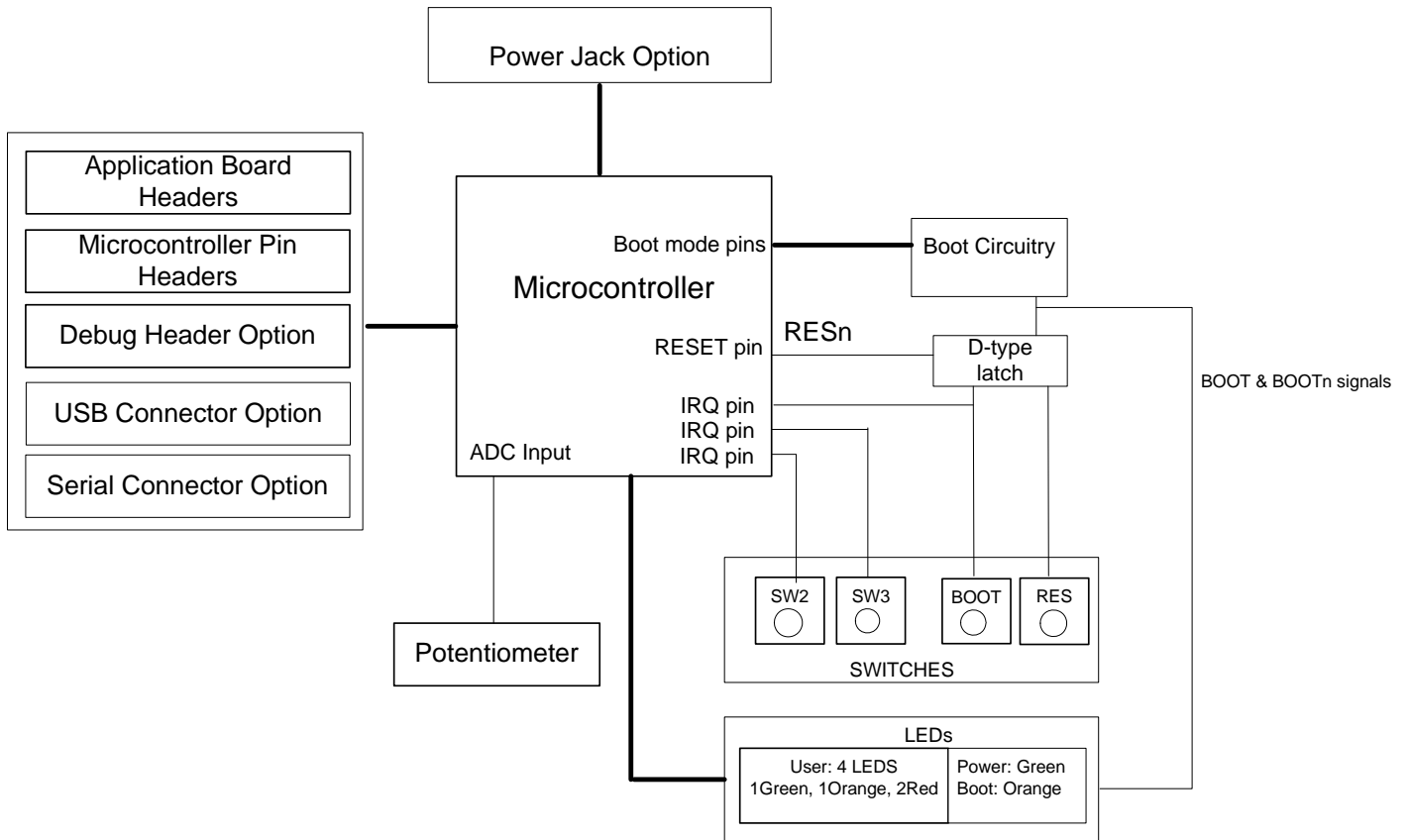
Figure 5-1: Block Diagram
