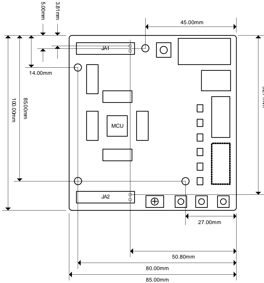
Figure 4-2 : Board Dimensions
