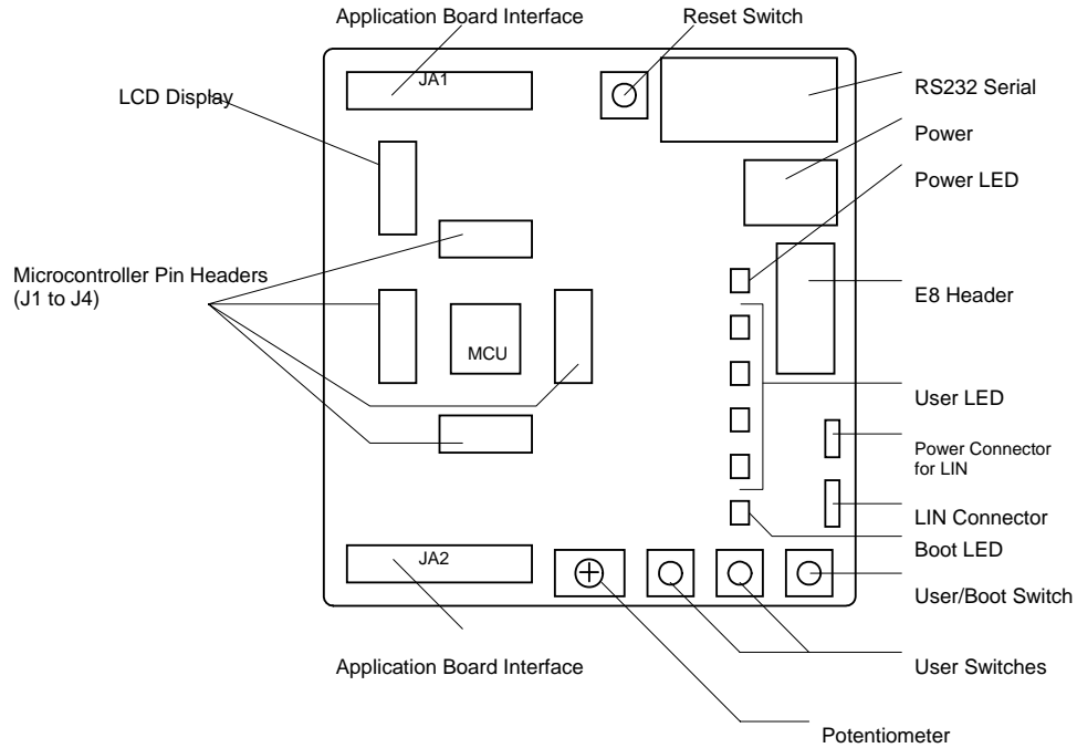
Figure 4-1: Board Layout
