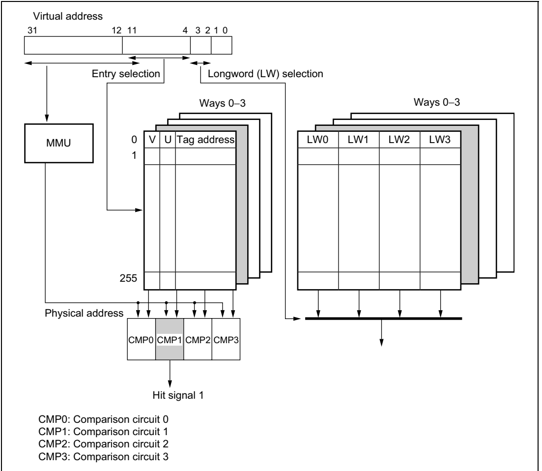
Figure 5.4 Cache Search Scheme (Normal Mode)
