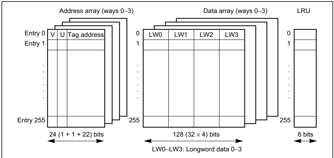
Figure 5.1 Cache Structure
