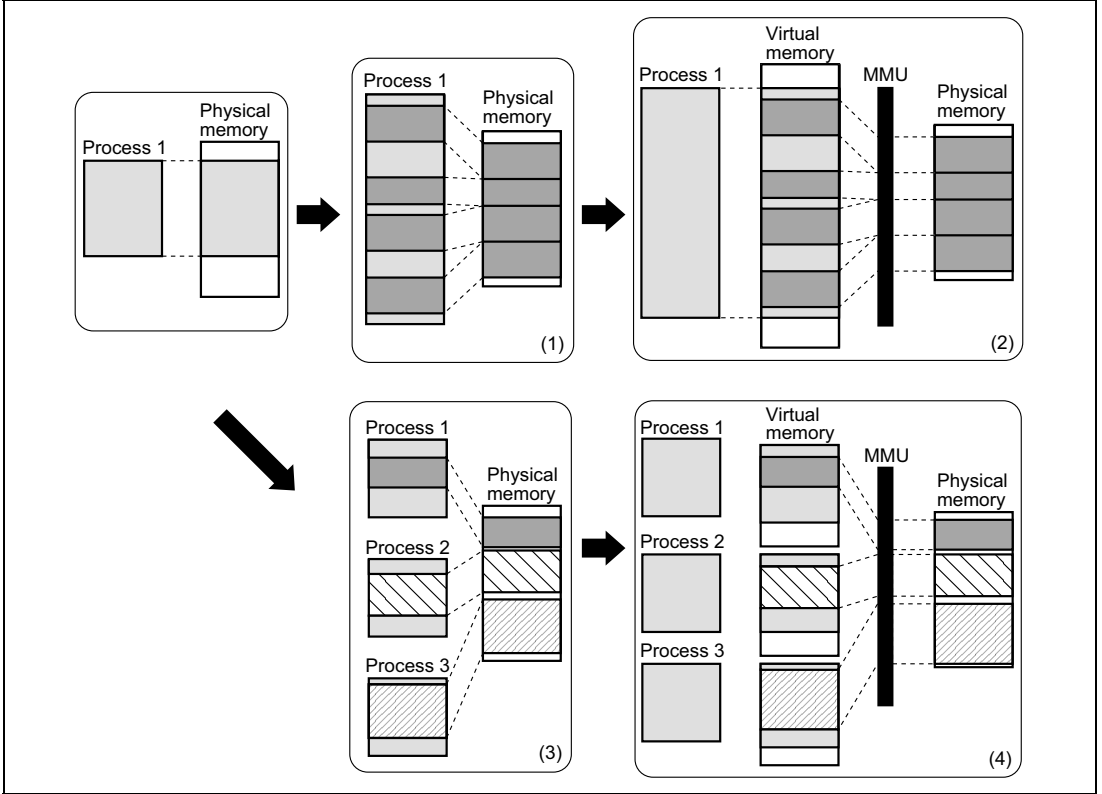
Figure 3.1 MMU Functions
