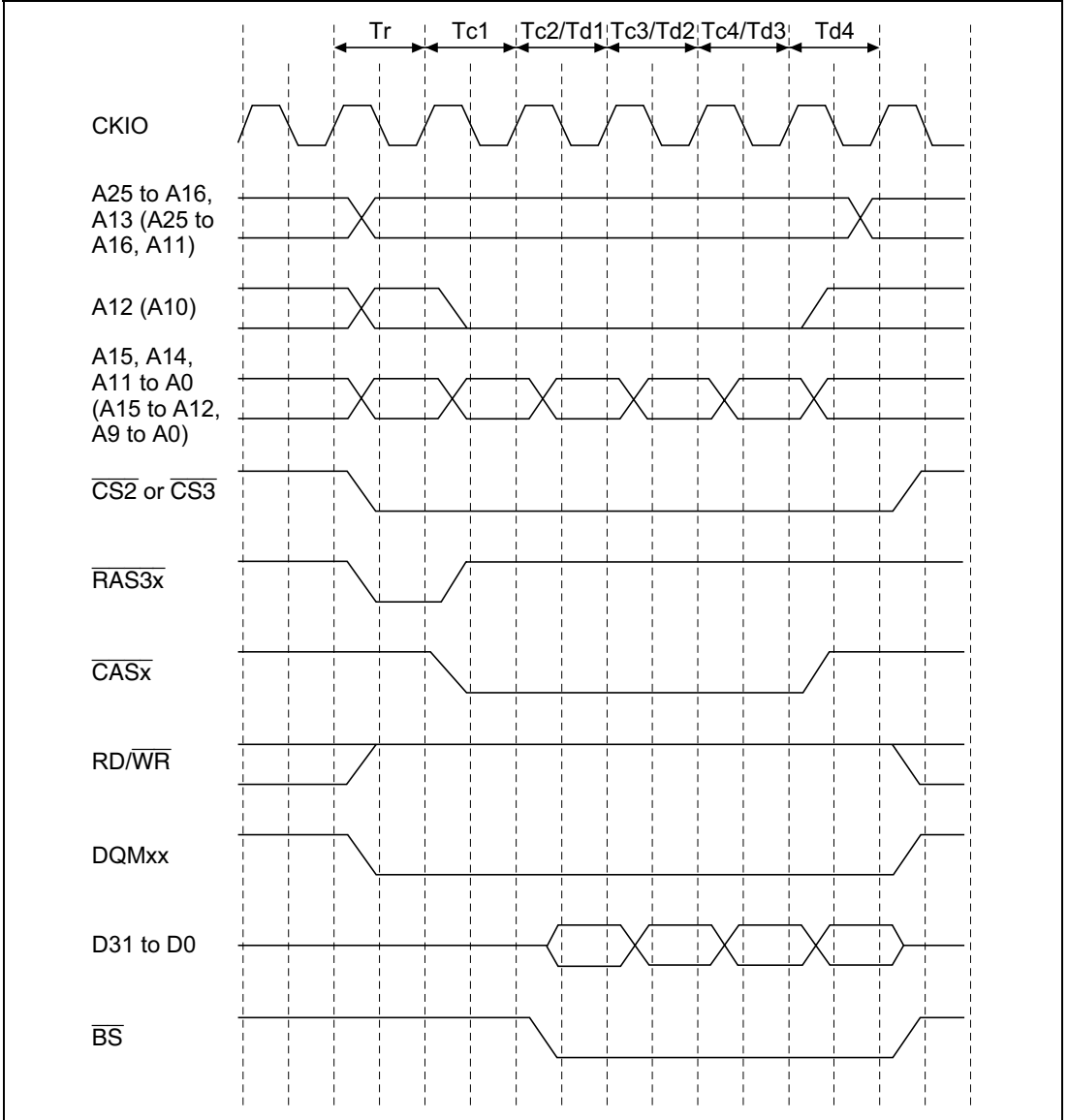
Figure 10.19 Burst Read Timing (No Precharge)
