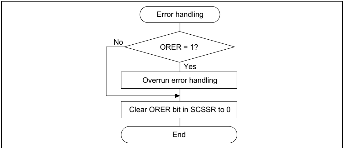
Figure 14.21 Sample Flowchart for Receiving Serial Data (cont)
