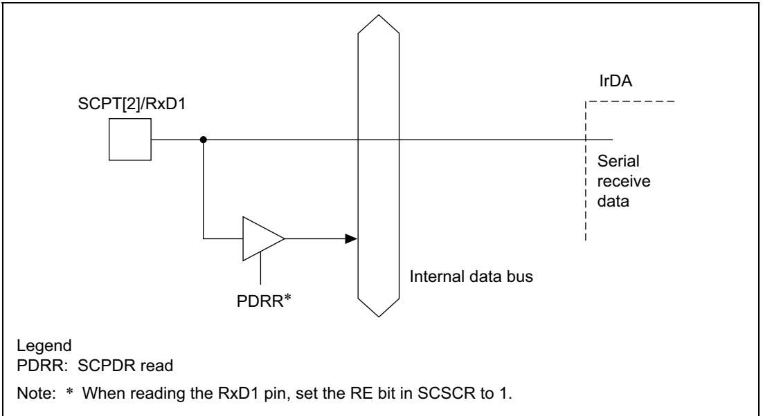
Figure 17.4 SCPT[2]/RxD1 Pin
