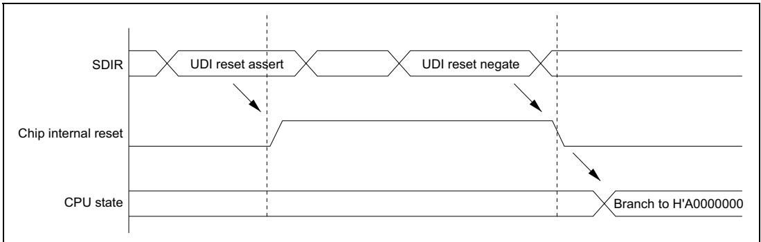
Figure 22.3 UDI Reset
