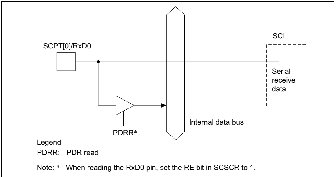
Figure 14.4 SCPT[0]/RxD0 Pin
