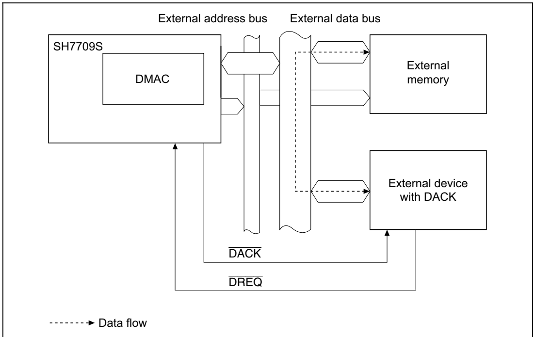
Figure 11.9 Data Flow in Single Address Mode
