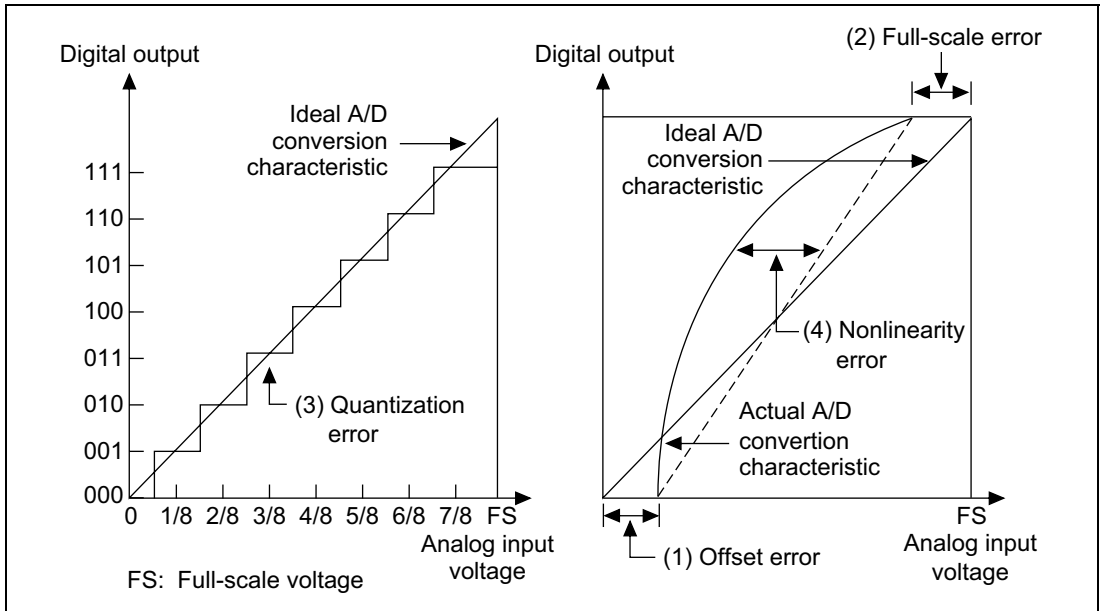
Figure 20.8 Definitions of A/D Conversion Accuracy
