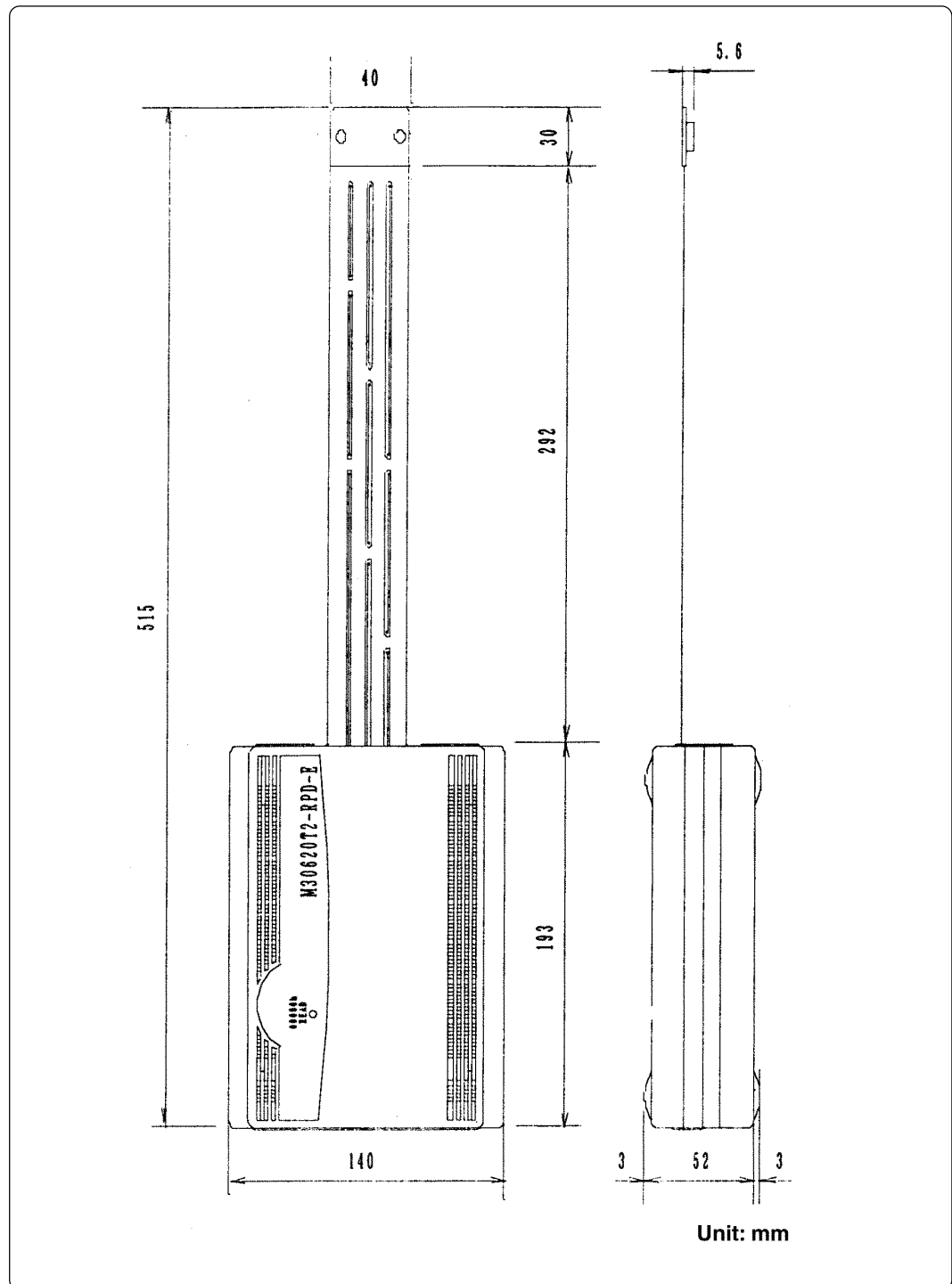
Figure 5.13 External dimensions of M30620T2-RPD-E
