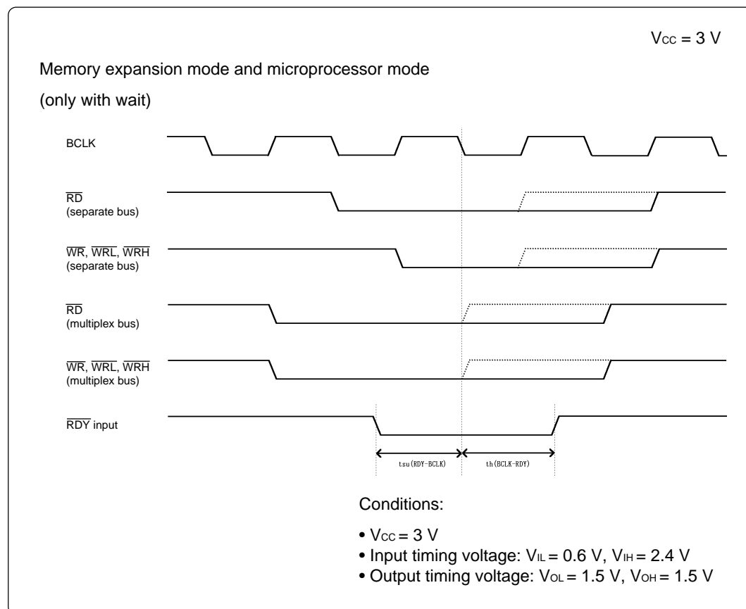
Figure 5.9 Timing requirements
