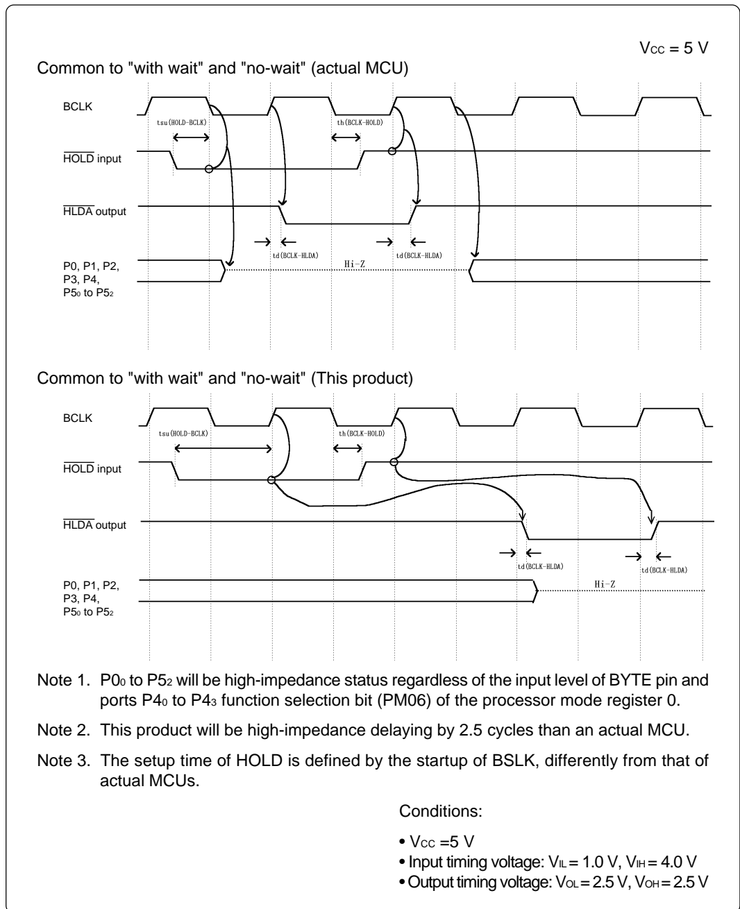
Figure 5.5 Timing requirements
