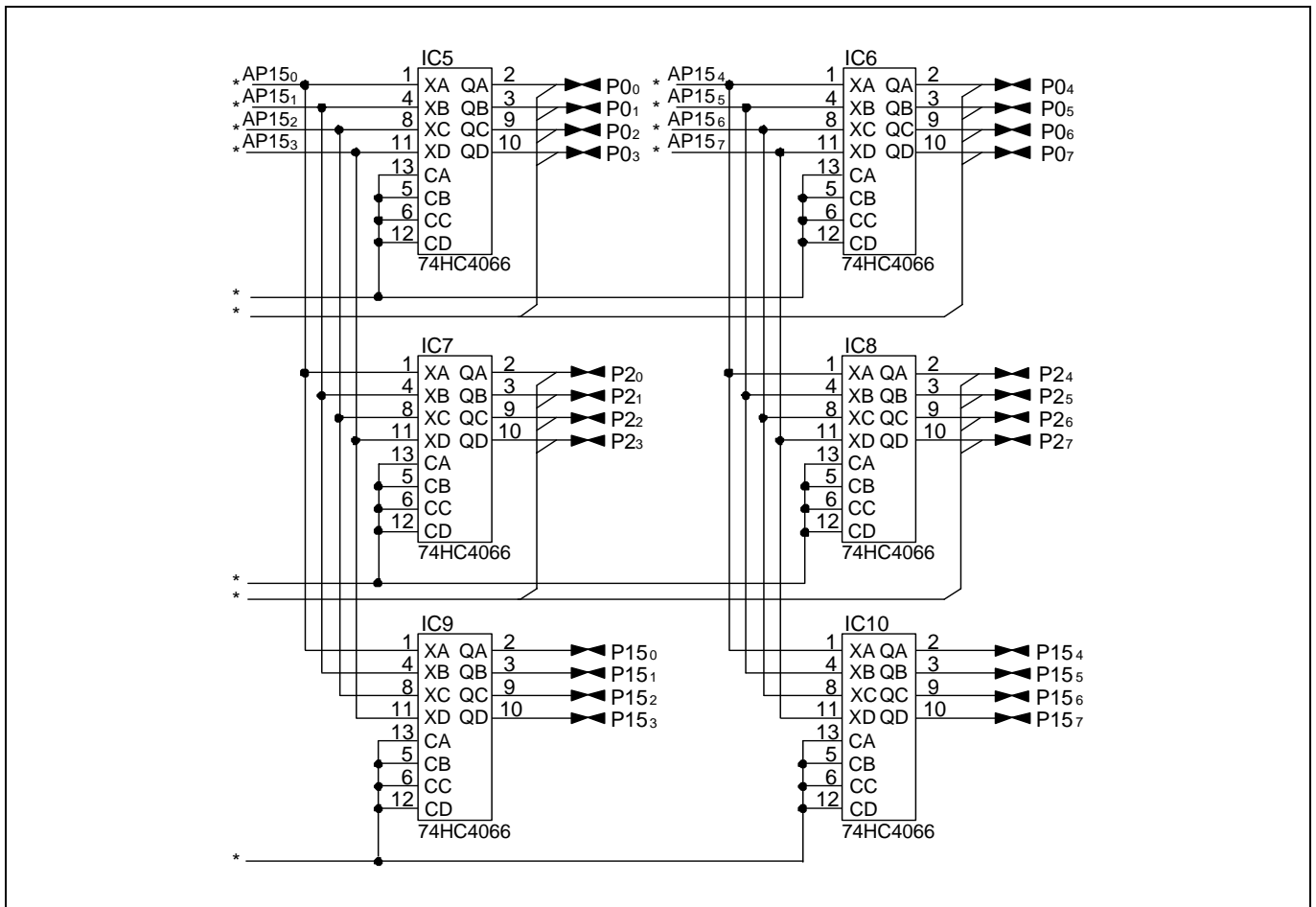
Figure 4.2 Connection diagram (2/2)
