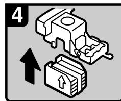
4 Push in the new refill until it clicks.
