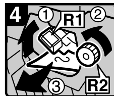
4 Hold up lever R1, turn knob R2, and then remove the misfed paper.
