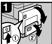
Open the bypass tray, and then open the duplex unit.
