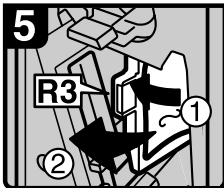
5 Open lever R3 to the left, and then remove the misfed paper.
