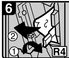
6 Push lever R4 to the right, and then remove the misfed paper.
