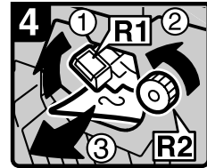
4 Hold up lever R1, turn knob R2, and then remove the misfed paper.
