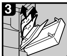
3 Remove the misfed paper.
