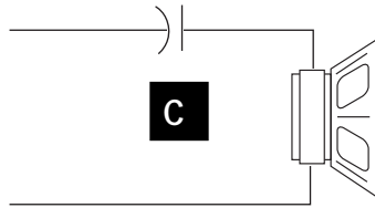
6dB/Octave High-Pass
