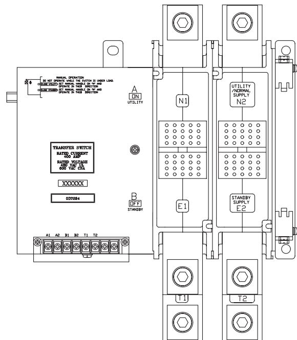
Figure 2.1 — Typical 2-Pole Transfer Mechanism (400 Amp Shown)
