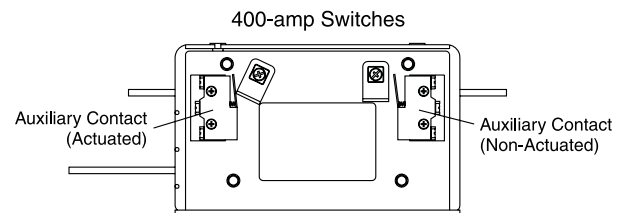
Figure 2.3 – Auxiliary Contacts
