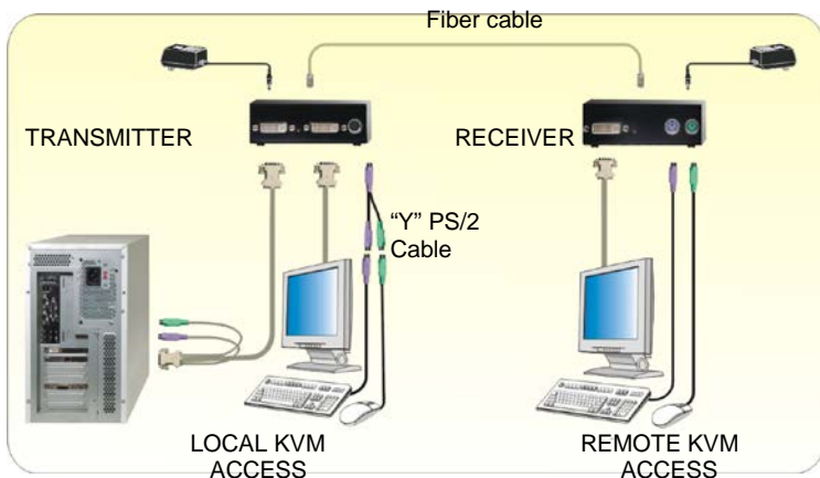
Figure 1. Typical cabling configurations
