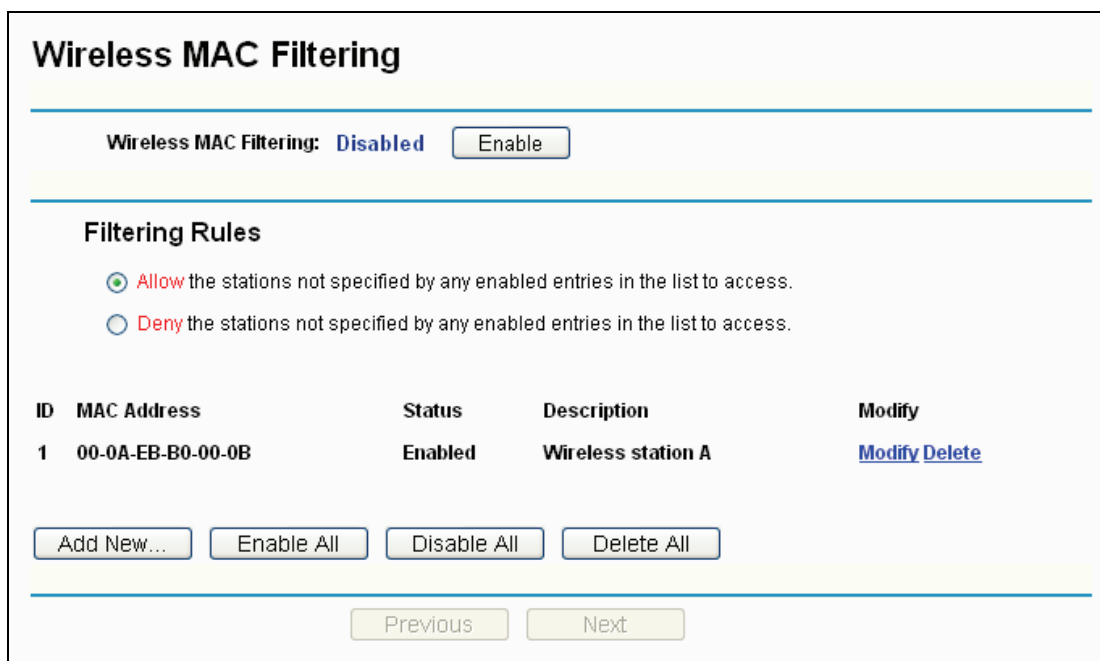
Figure 4-22 Wireless MAC Filtering
