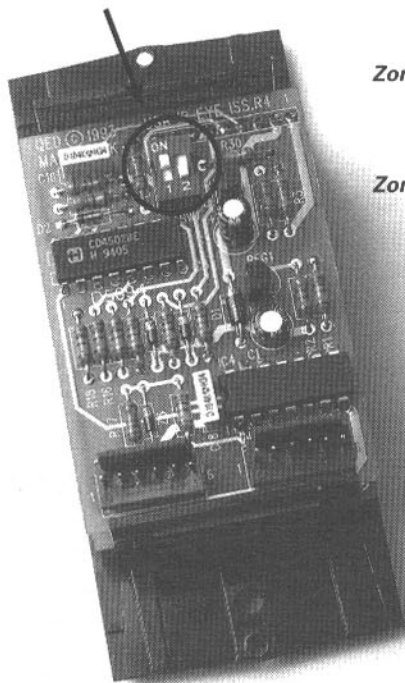
Zone switches
