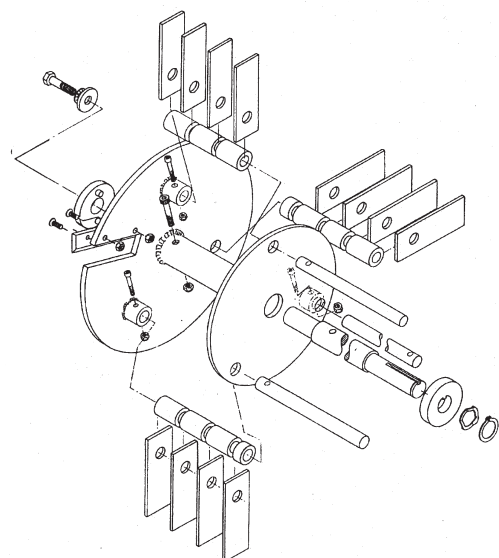
Figure 12. Rotor assembly
