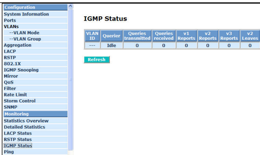
Fig. 4-32 IGMP Status
