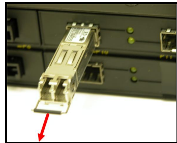
Figure 29: SFP Removal
