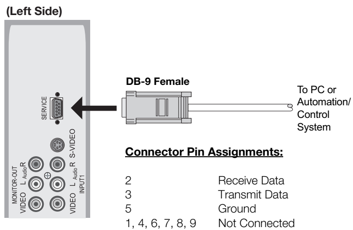
Figure 3-8. RS-232 Control System Connection
