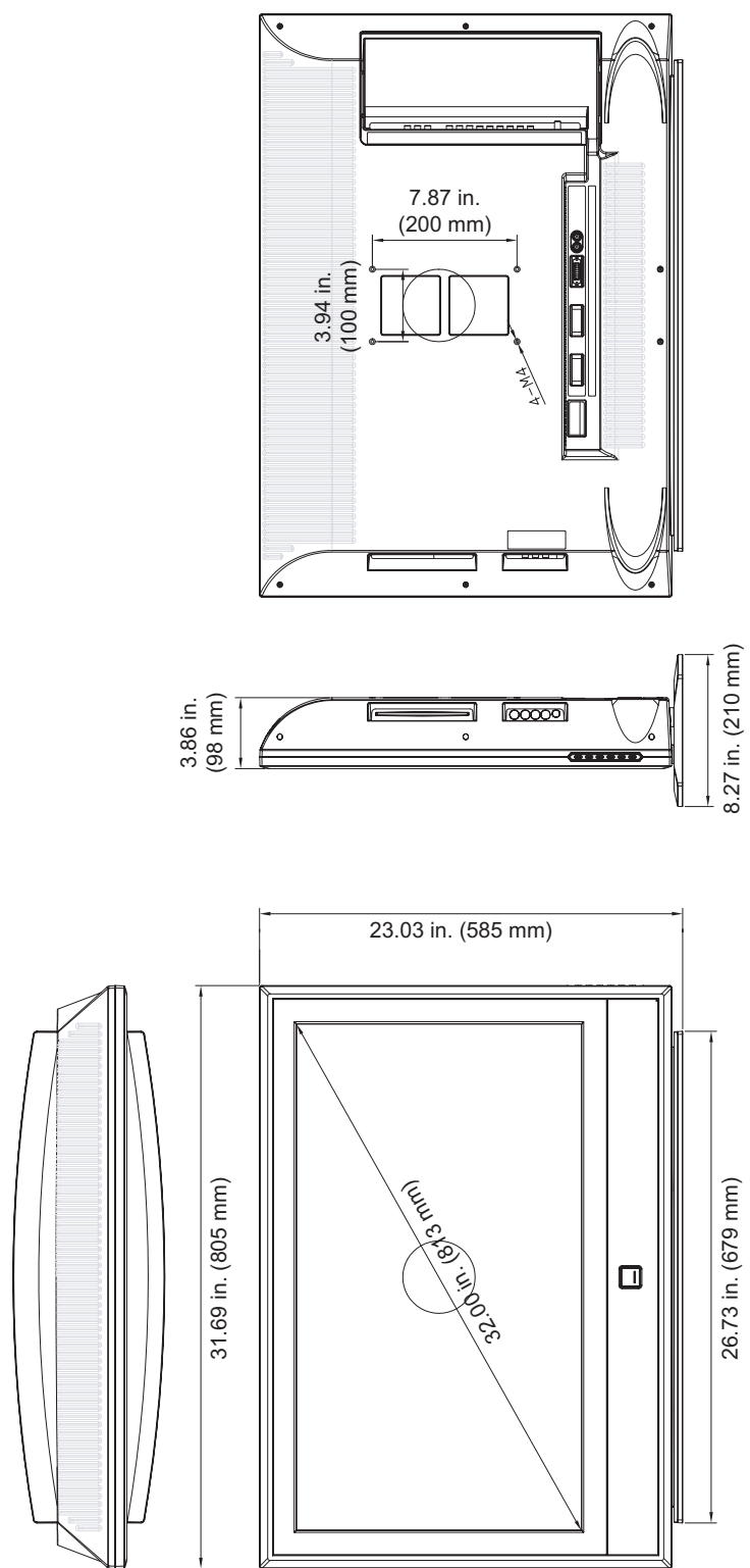
Figure 7-2. CR-32HDi Dimensions
