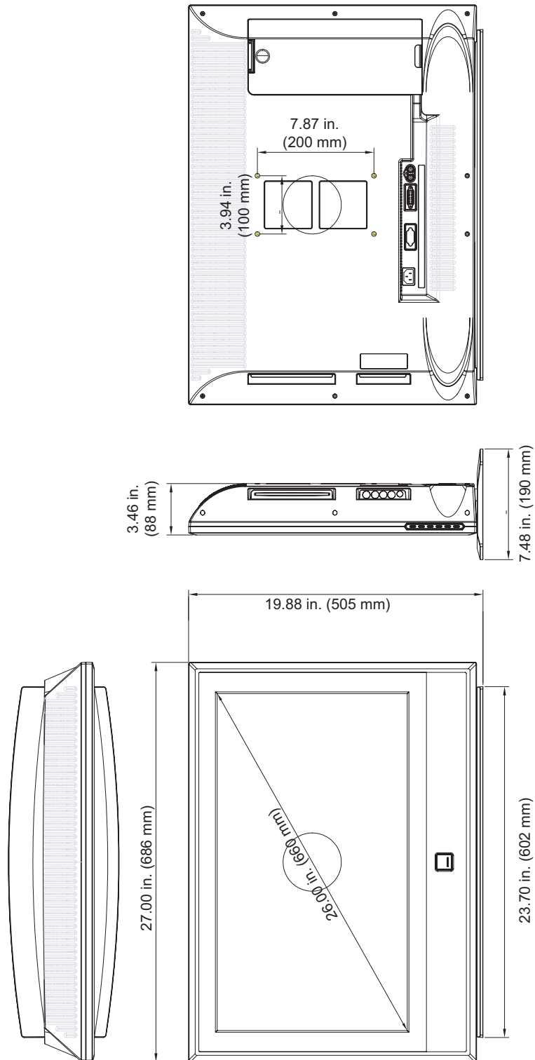
Figure 7-1. CR-26HD Dimensions
