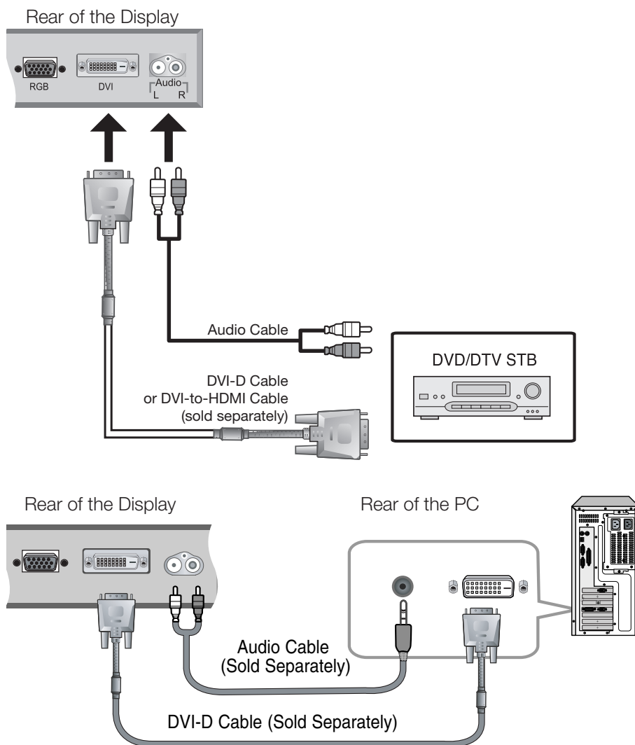
Figure 3-2. DVI Connections
