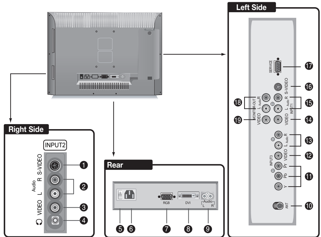
Figure 2-2. Crystal Series LCD Display Rear-Panel Inputs and Outputs
