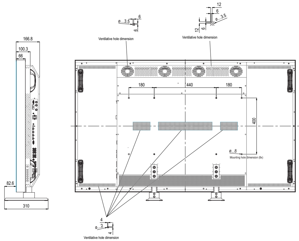
Figure 7-4. CX-65HD Overall Dimensions (Rear/Side)
