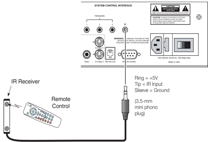
Figure 3-13. External IR Receiver Connection
