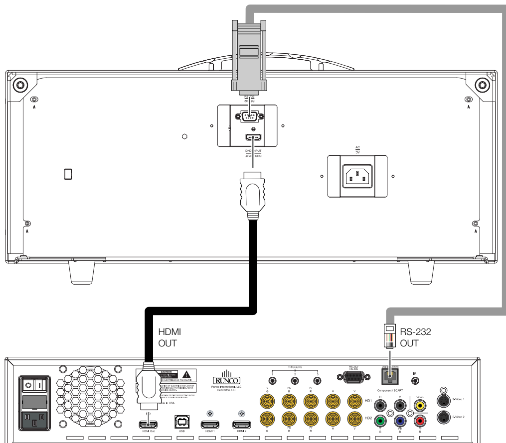
Figure 3-10. Connecting the Q-750d to the DHD Controller
