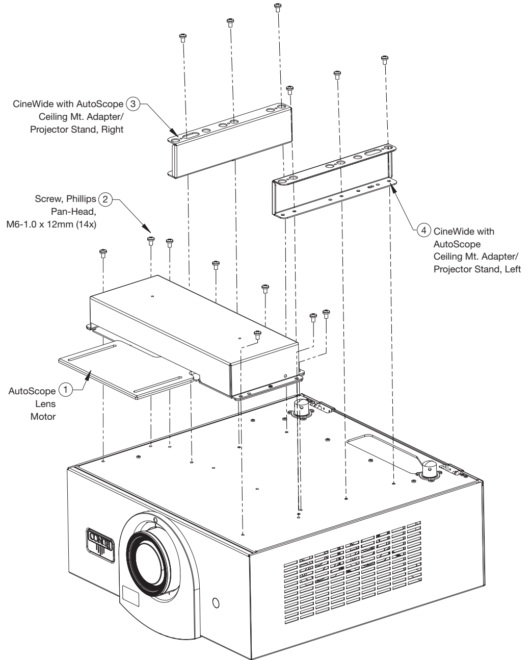
Figure 3-6. Q-750i/CineWide with AutoScope Motor Assembly
