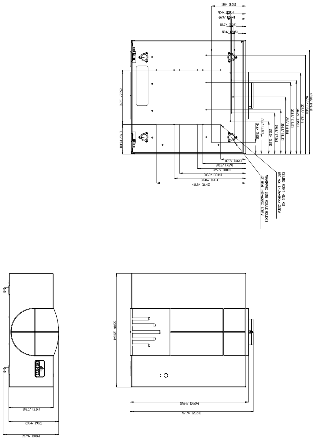
Figure 7-1. Overall Dimensions – Q-750i
