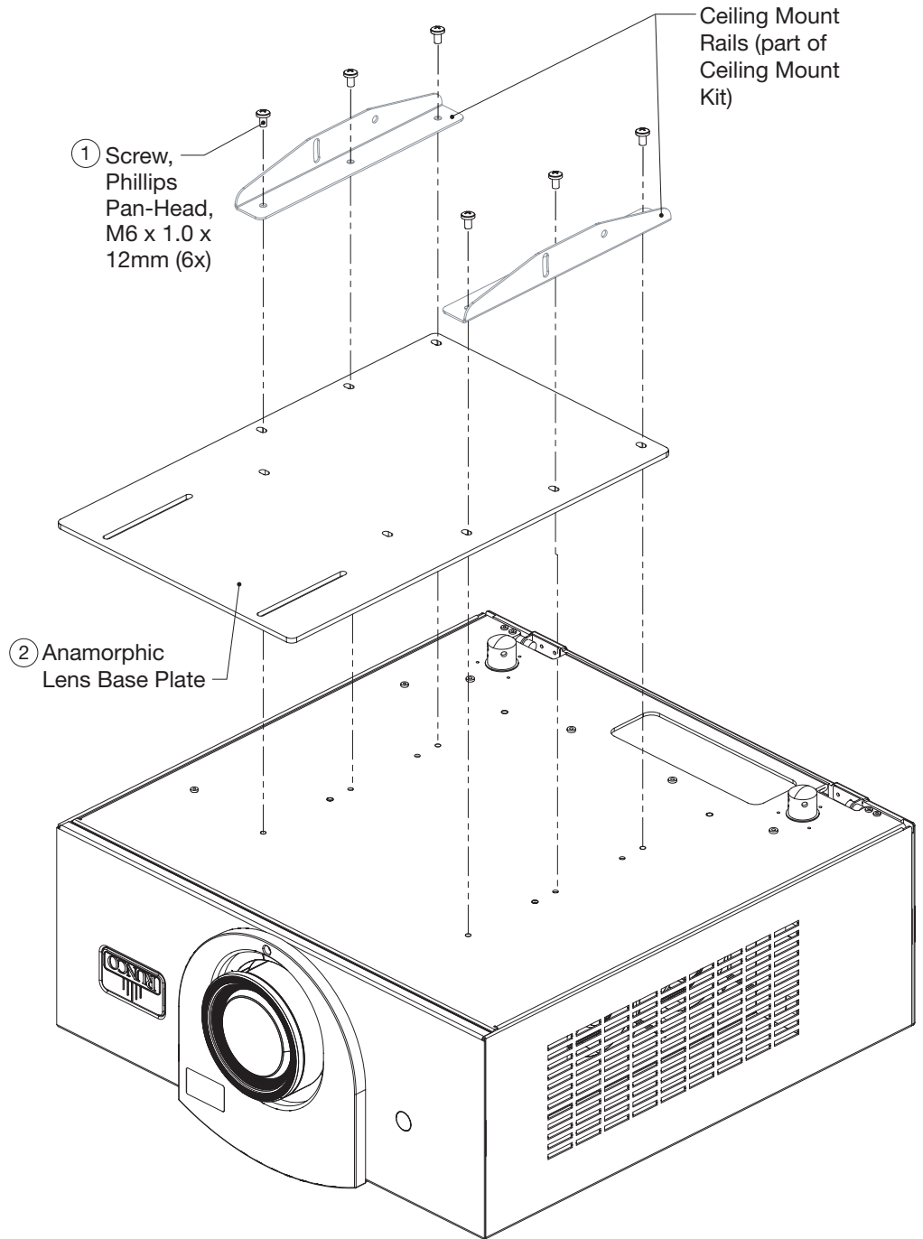
Figure 3-9. Q-750i/CineWide with Rainier II/McKinley (Cylindrical) Lens Base Plate - Exploded View
