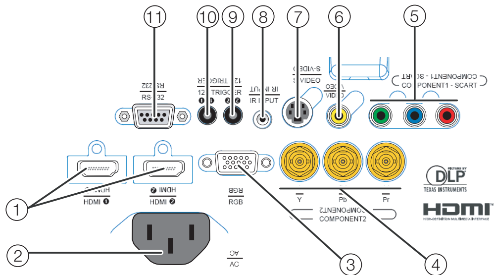
Figure 2-2. Q-750i Rear Panel
