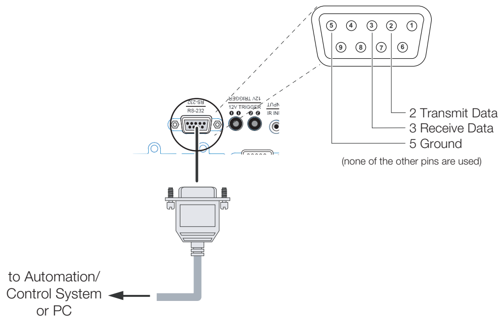
Figure 3-14. RS-232 Control System Connection
