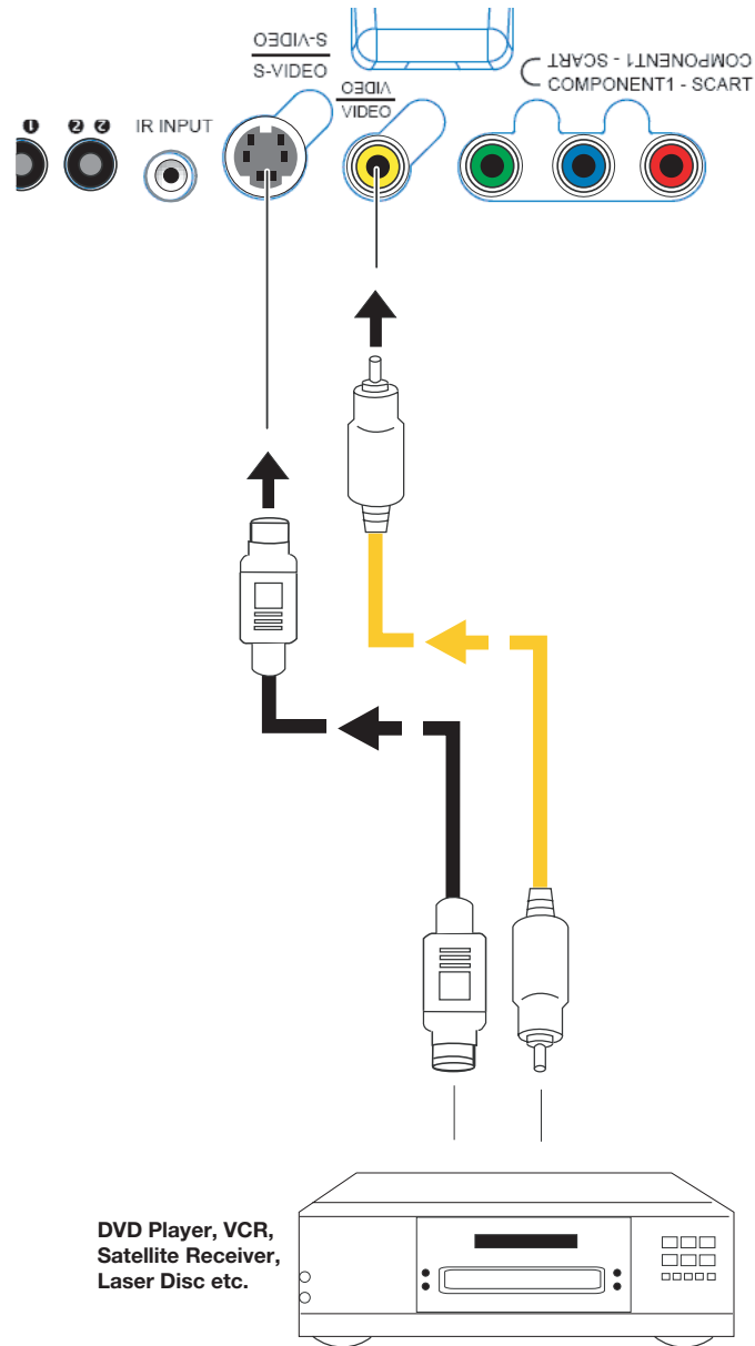
Figure 3-13. Composite and S-Video Connections
