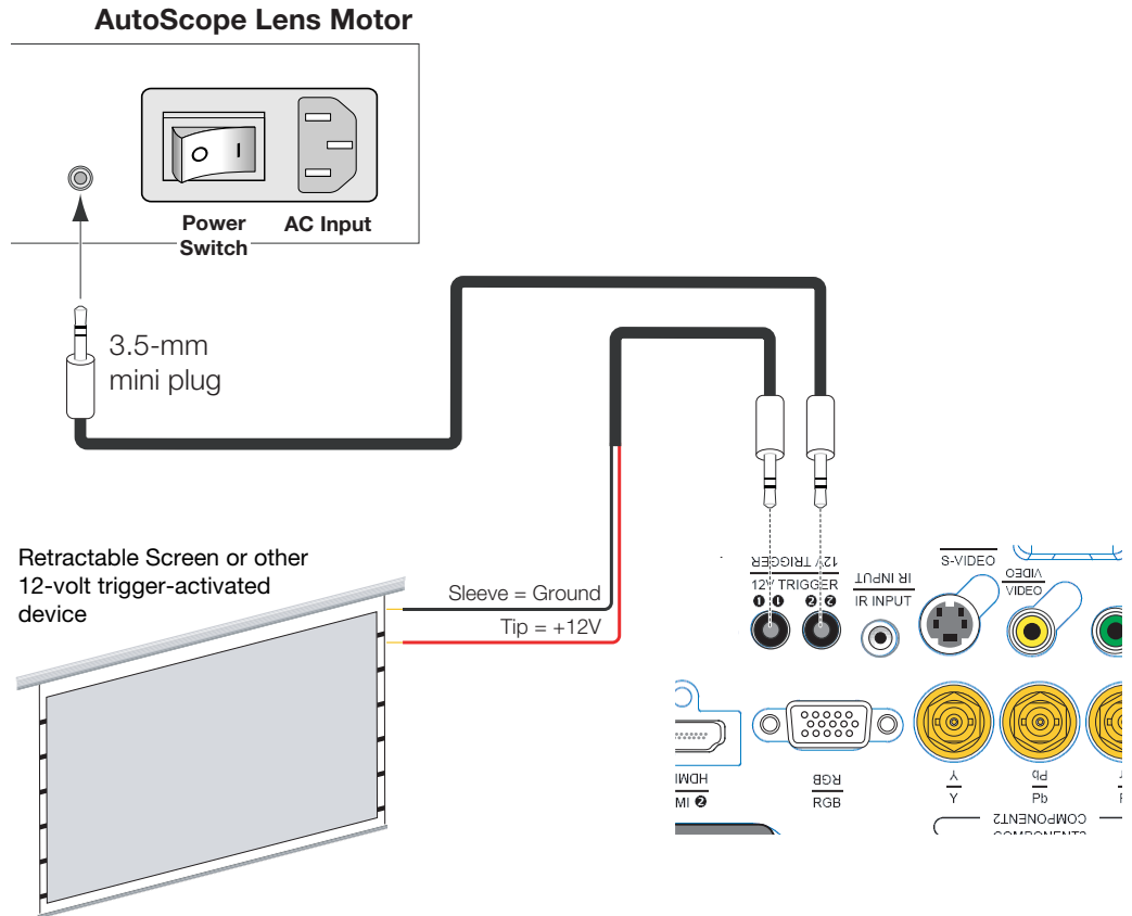
Figure 3-15. Connecting 12-Volt Trigger Outputs
