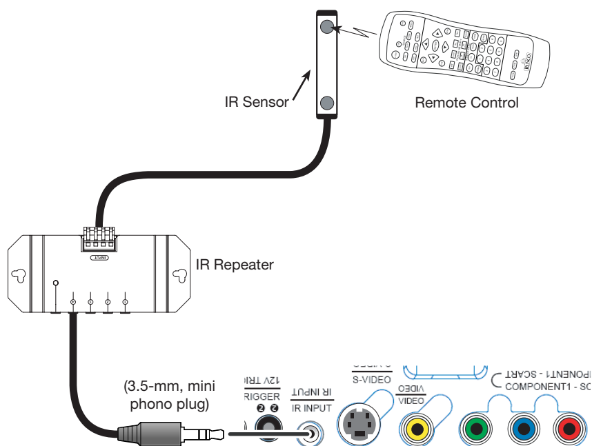
Figure 3-16. External IR Receiver Connection
