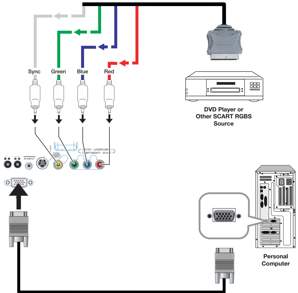
Figure 3-11. RGB Connections
