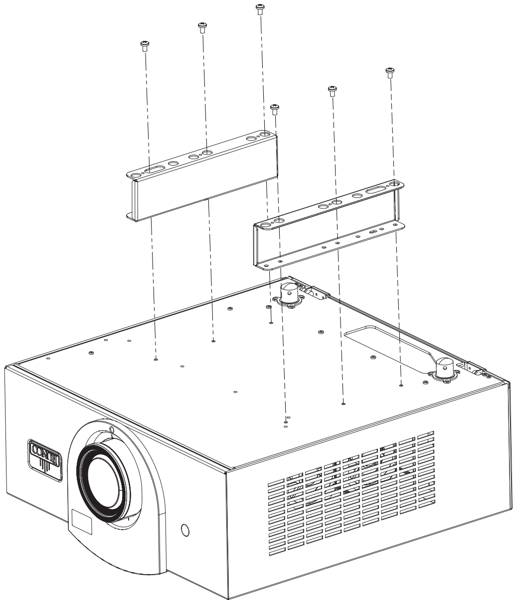
Figure 3-7. Q750i with Ceiling Mount Adapters/Projector Stands
