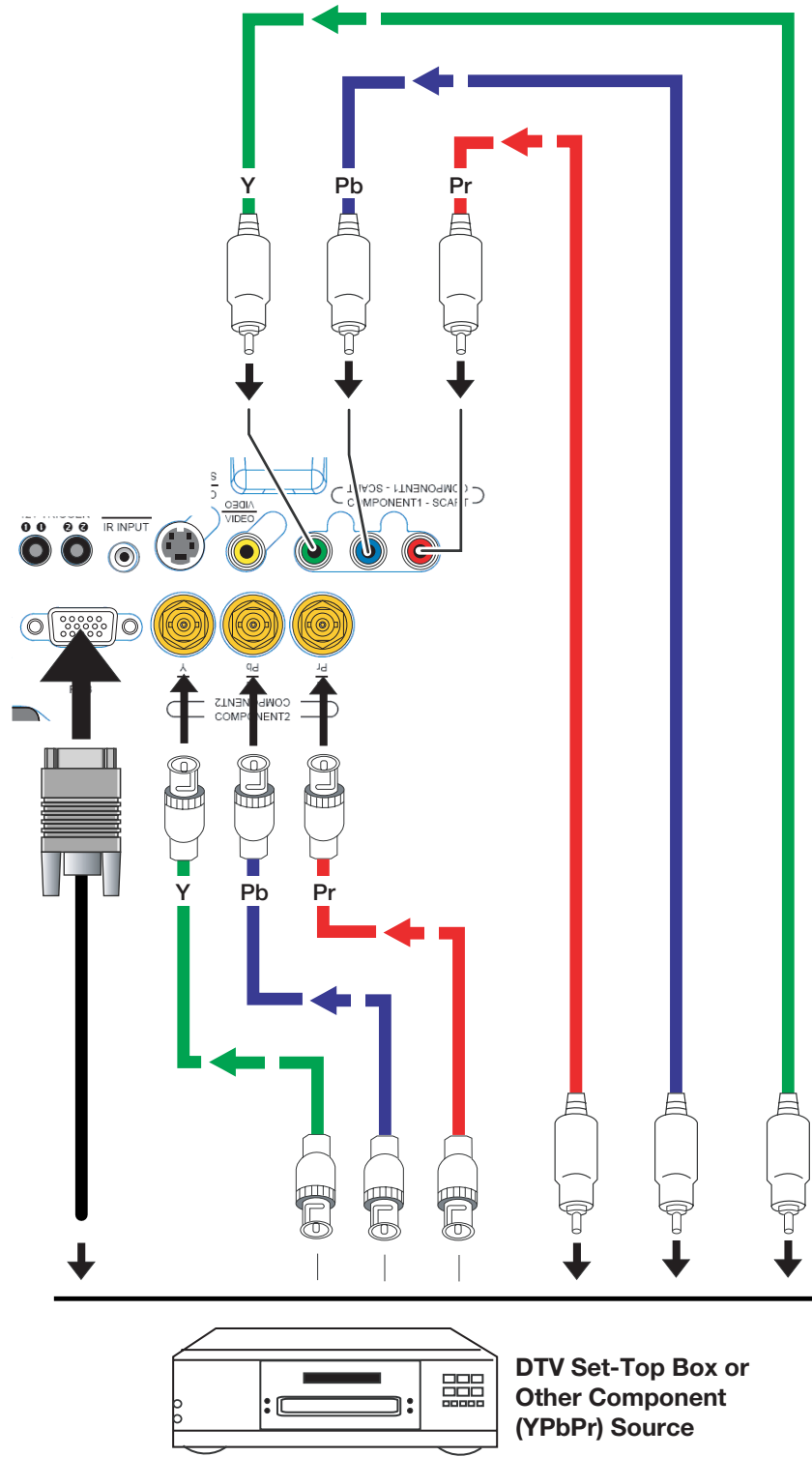
Figure 3-12. Component Video Connections
