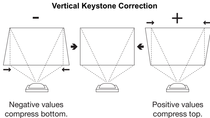
Figure 4-6. Keystone Correction
