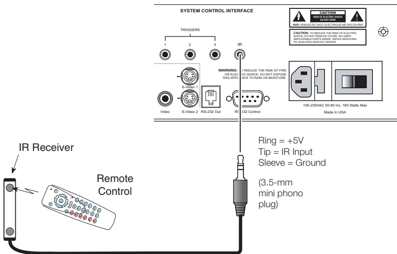
Figure 3-15. External IR Receiver Connection
