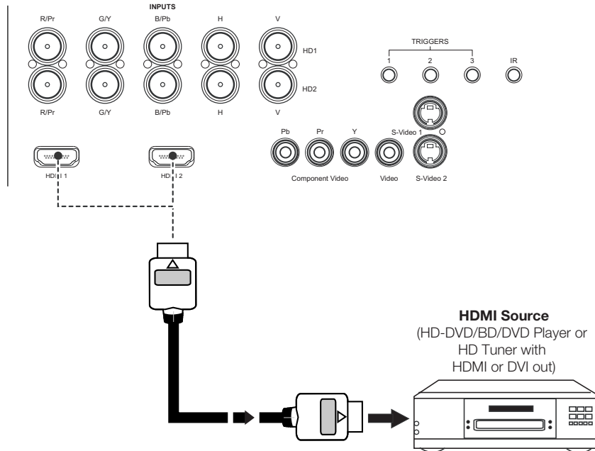
Figure 3-9. HDMI Source Connections
