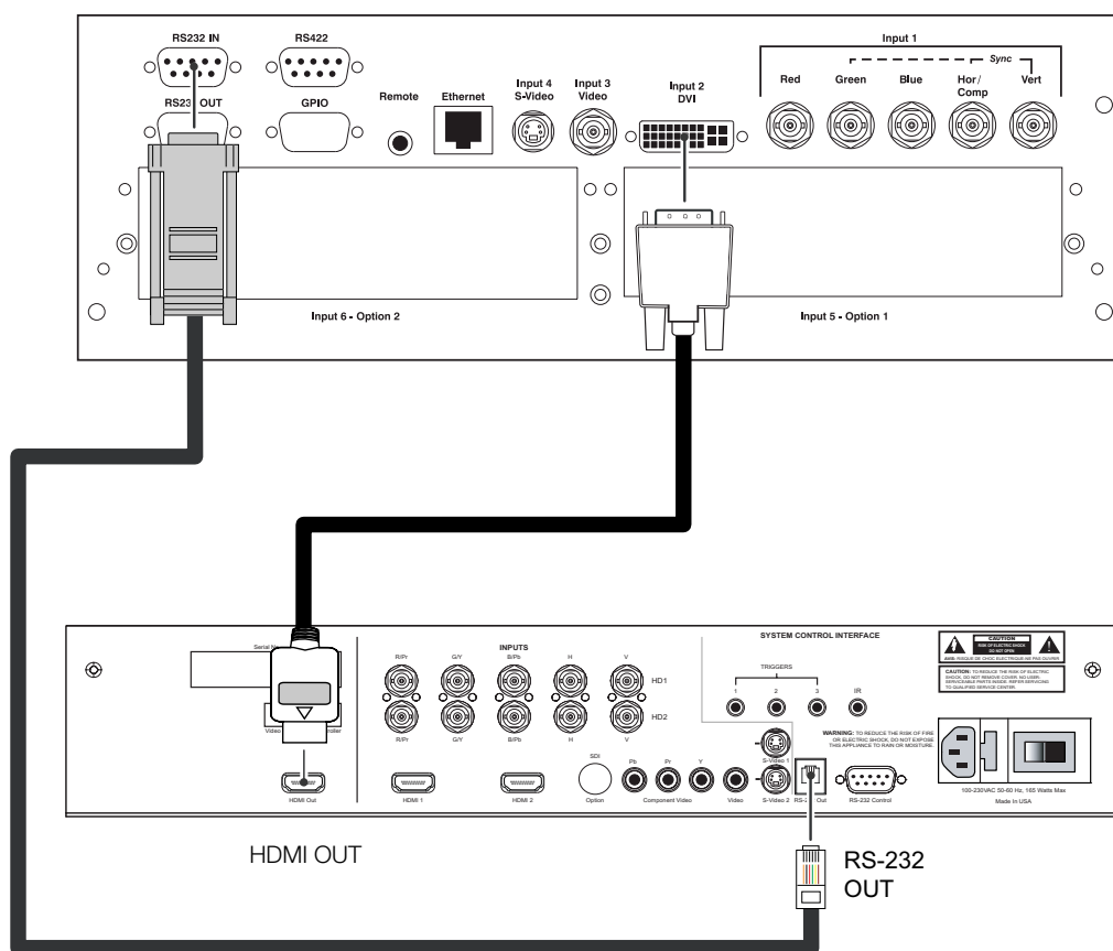
Figure 3-8. Connecting the VX-44d/-55d to the DHD Controller
