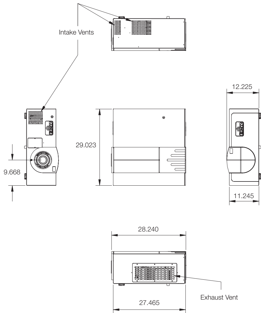
Figure 7-1. VX-44d/-55d Dimensions
