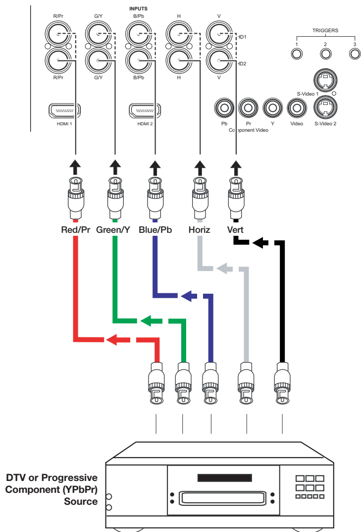
Figure 3-10. Digital (DTV) RGB or Component Video Connections
