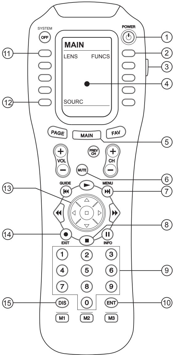
Figure 3-16. TheaterMaster Remote Control for VX-44d/-55d
