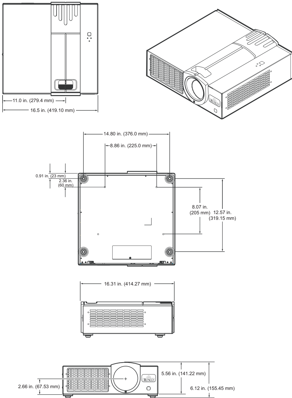
Figure 7-1. CL-610 Dimensions
