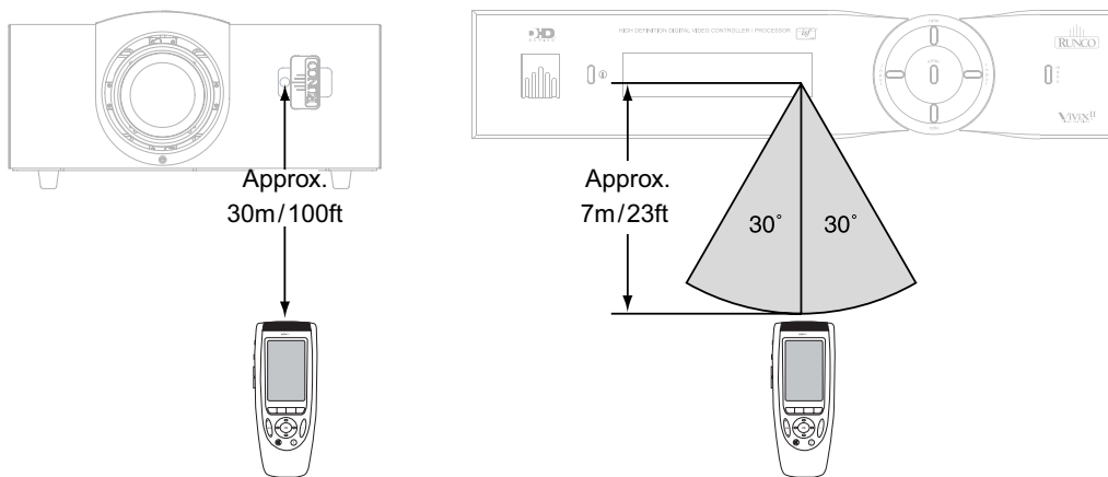
Figure 3-1. Available Range of the Remote Control
