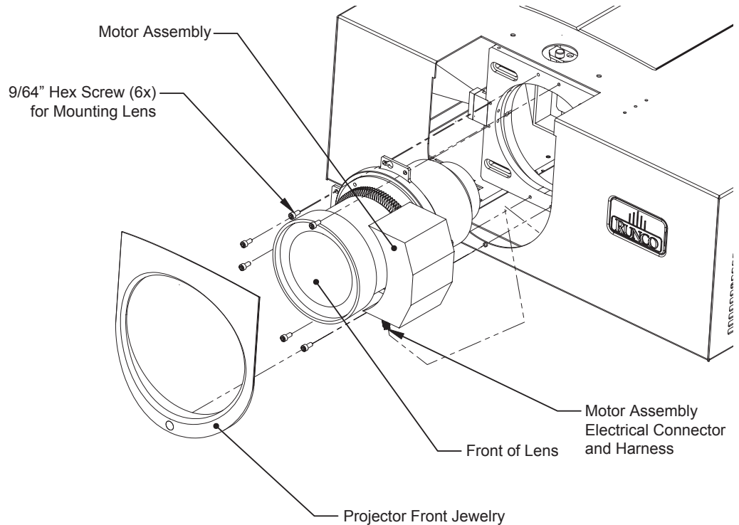
Figure 5-1. VX-5000d Lens Assembly Exploded View
